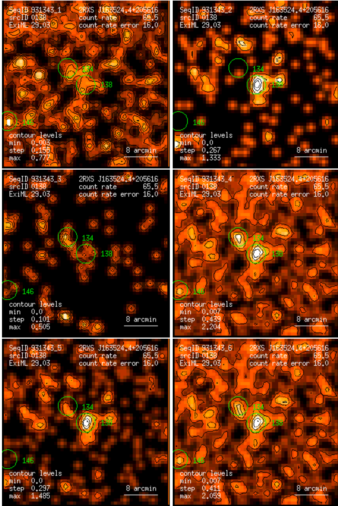
Figure 138: RASS 931343: detection 0138: band rate images, Gaussian filter: (1) PSPC channels 11 – 41, (2) 52 – 90, (3) 91 – 201, (4) 11 – 235, (5) 52 – 201, (6) 11 – 201. Broad band rates in counts/ks. Band rate contour levels in counts/ks/arcmin 2 .
