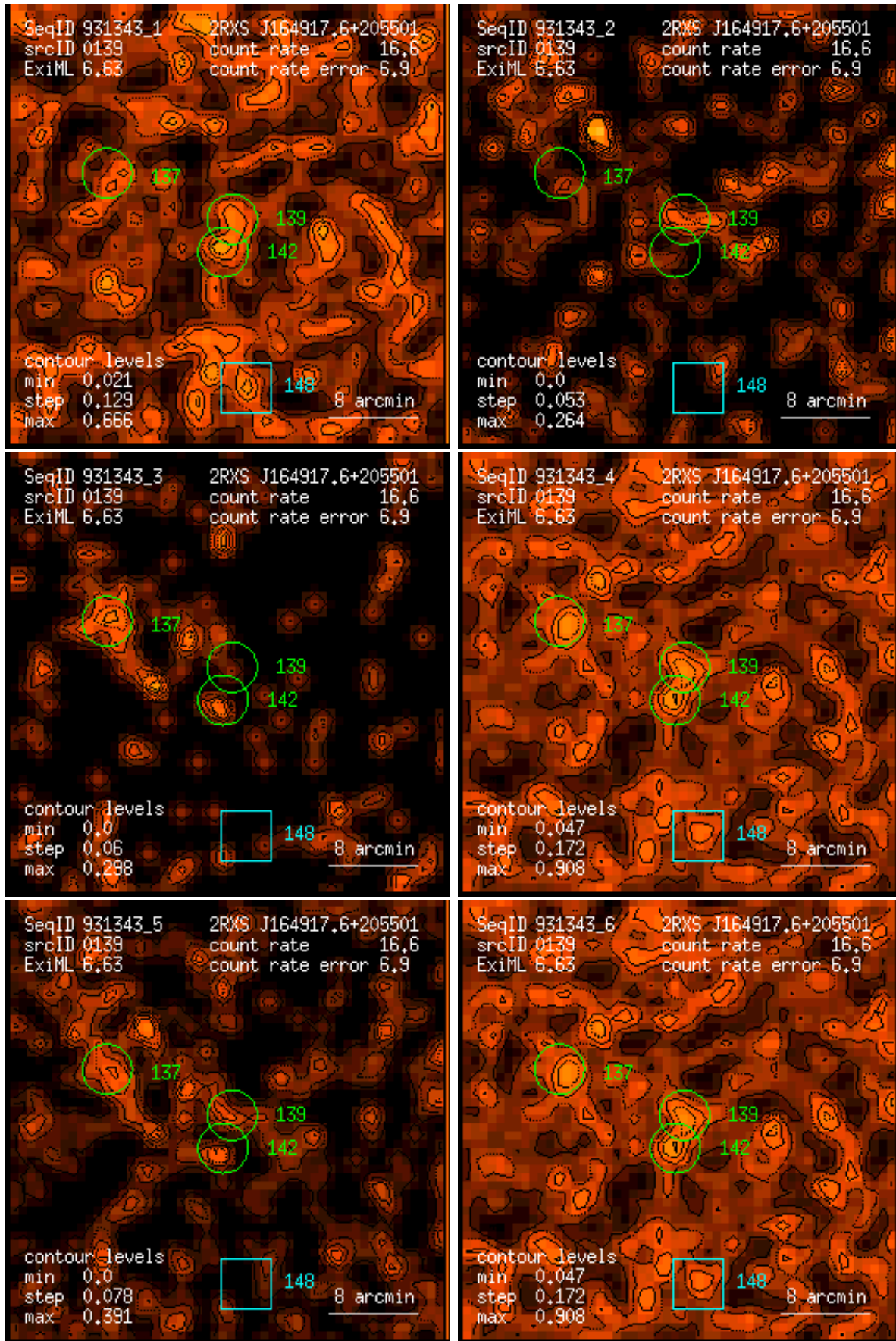
Figure 139: RASS 931343: detection 0139: band rate images, Gaussian filter: (1) PSPC channels 11 – 41, (2) 52 – 90, (3) 91 – 201, (4) 11 – 235, (5) 52 – 201, (6) 11 – 201. Broad band rates in counts/ks. Band rate contour levels in counts/ks/arcmin 2 .
