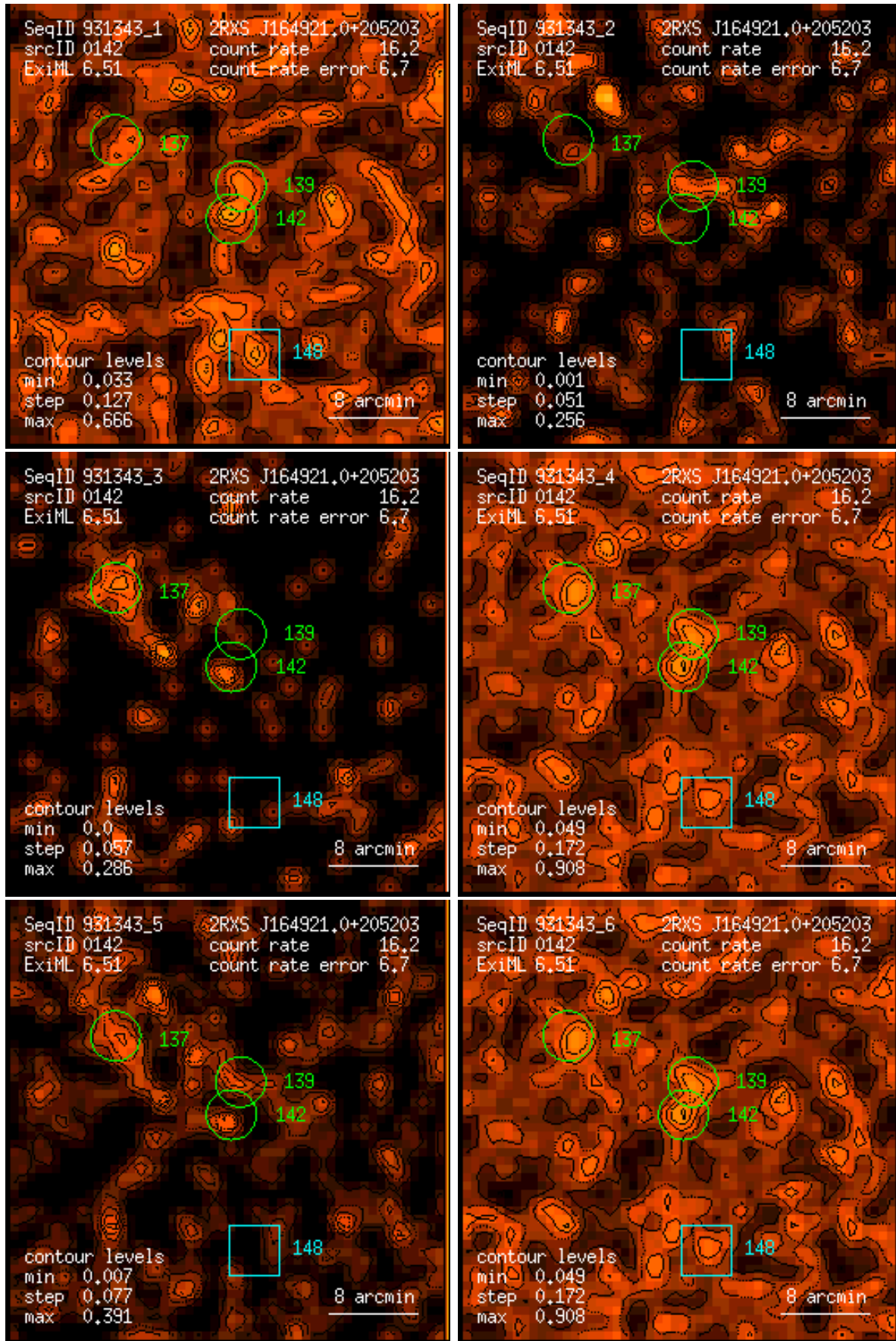
Figure 142: RASS 931343: detection 0142: band rate images, Gaussian filter: (1) PSPC channels 11 – 41, (2) 52 – 90, (3) 91 – 201, (4) 11 – 235, (5) 52 – 201, (6) 11 – 201. Broad band rates in counts/ks. Band rate contour levels in counts/ks/arcmin 2 .
