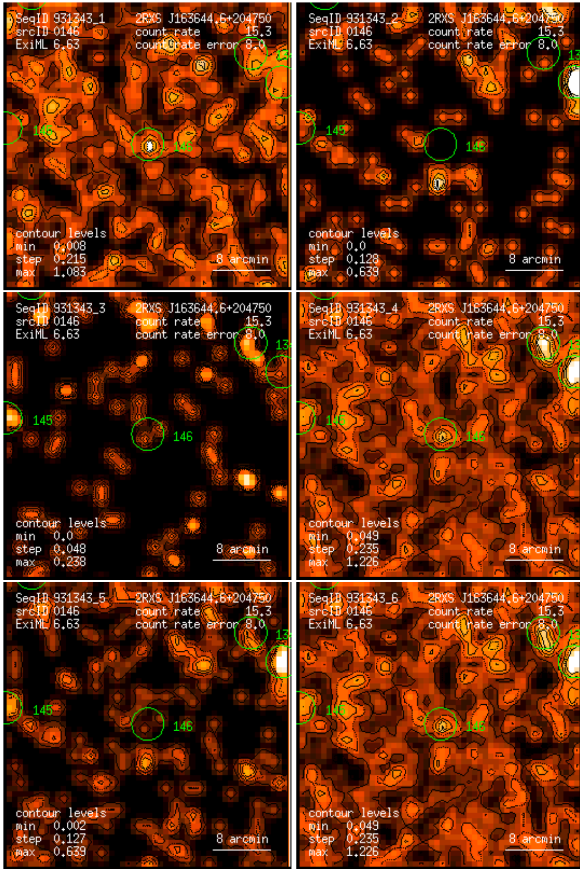
Figure 146: RASS 931343: detection 0146: band rate images, Gaussian filter: (1) PSPC channels 11 – 41, (2) 52 – 90, (3) 91 – 201, (4) 11 – 235, (5) 52 – 201, (6) 11 – 201. Broad band rates in counts/ks. Band rate contour levels in counts/ks/arcmin 2 .
