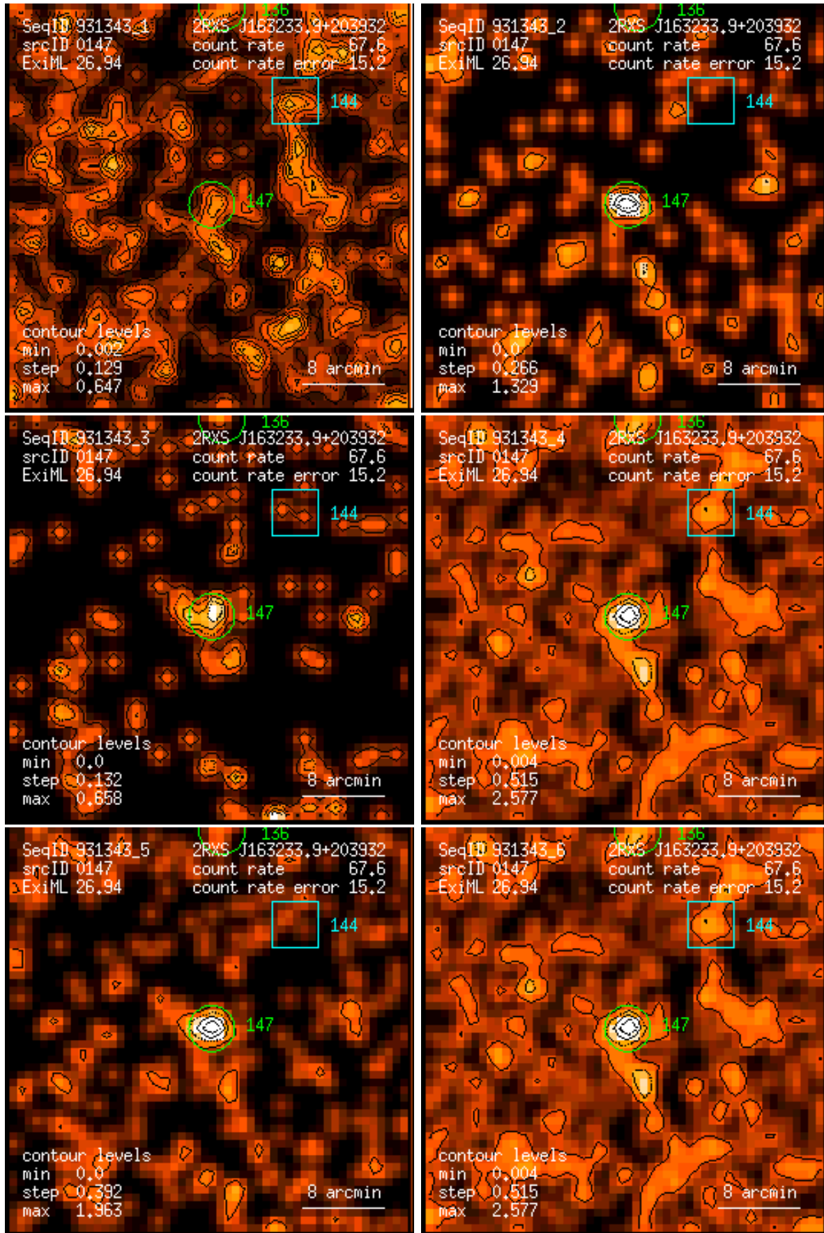
Figure 147: RASS 931343: detection 0147: band rate images, Gaussian filter: (1) PSPC channels 11 – 41, (2) 52 – 90, (3) 91 – 201, (4) 11 – 235, (5) 52 – 201, (6) 11 – 201. Broad band rates in counts/ks. Band rate contour levels in counts/ks/arcmin 2 .
