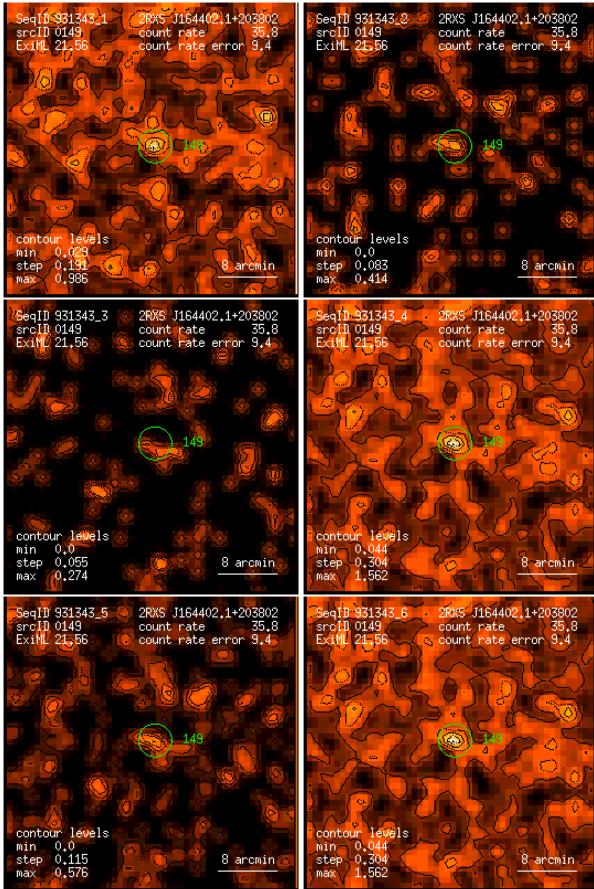
Figure 149: RASS 931343: detection 0149: band rate images, Gaussian filter: (1) PSPC channels 11 – 41, (2) 52 – 90, (3) 91 – 201, (4) 11 – 235, (5) 52 – 201, (6) 11 – 201. Broad band rates in counts/ks. Band rate contour levels in counts/ks/arcmin 2 .
