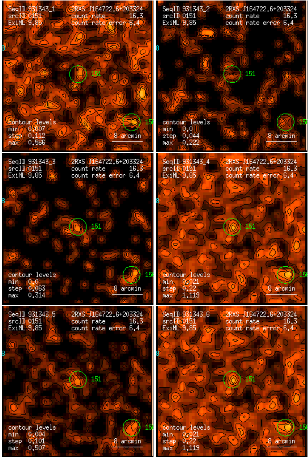
Figure 151: RASS 931343: detection 0151: band rate images, Gaussian filter: (1) PSPC channels 11 – 41, (2) 52 – 90, (3) 91 – 201, (4) 11 – 235, (5) 52 – 201, (6) 11 – 201. Broad band rates in counts/ks. Band rate contour levels in counts/ks/arcmin 2 .
