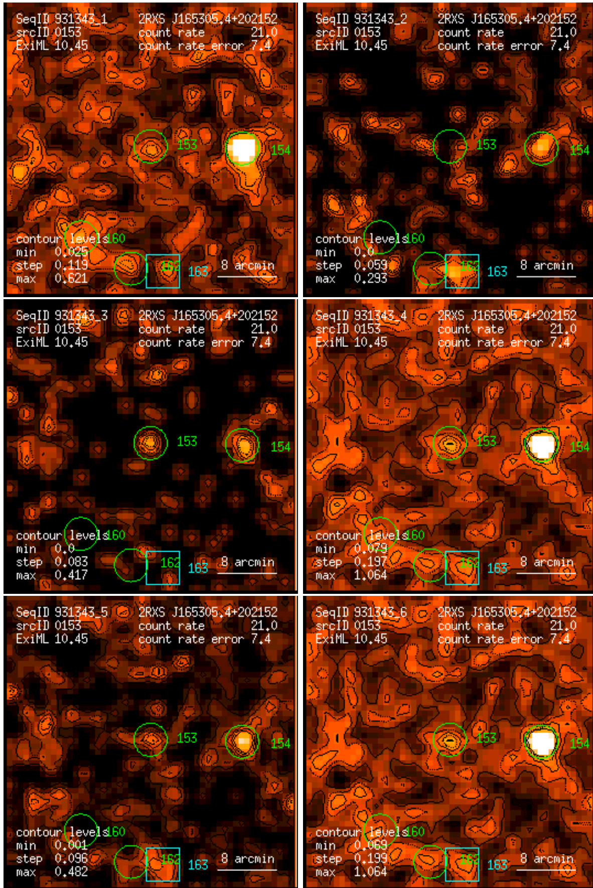
Figure 153: RASS 931343: detection 0153: band rate images, Gaussian filter: (1) PSPC channels 11 – 41, (2) 52 – 90, (3) 91 – 201, (4) 11 – 235, (5) 52 – 201, (6) 11 – 201. Broad band rates in counts/ks. Band rate contour levels in counts/ks/arcmin 2 .
