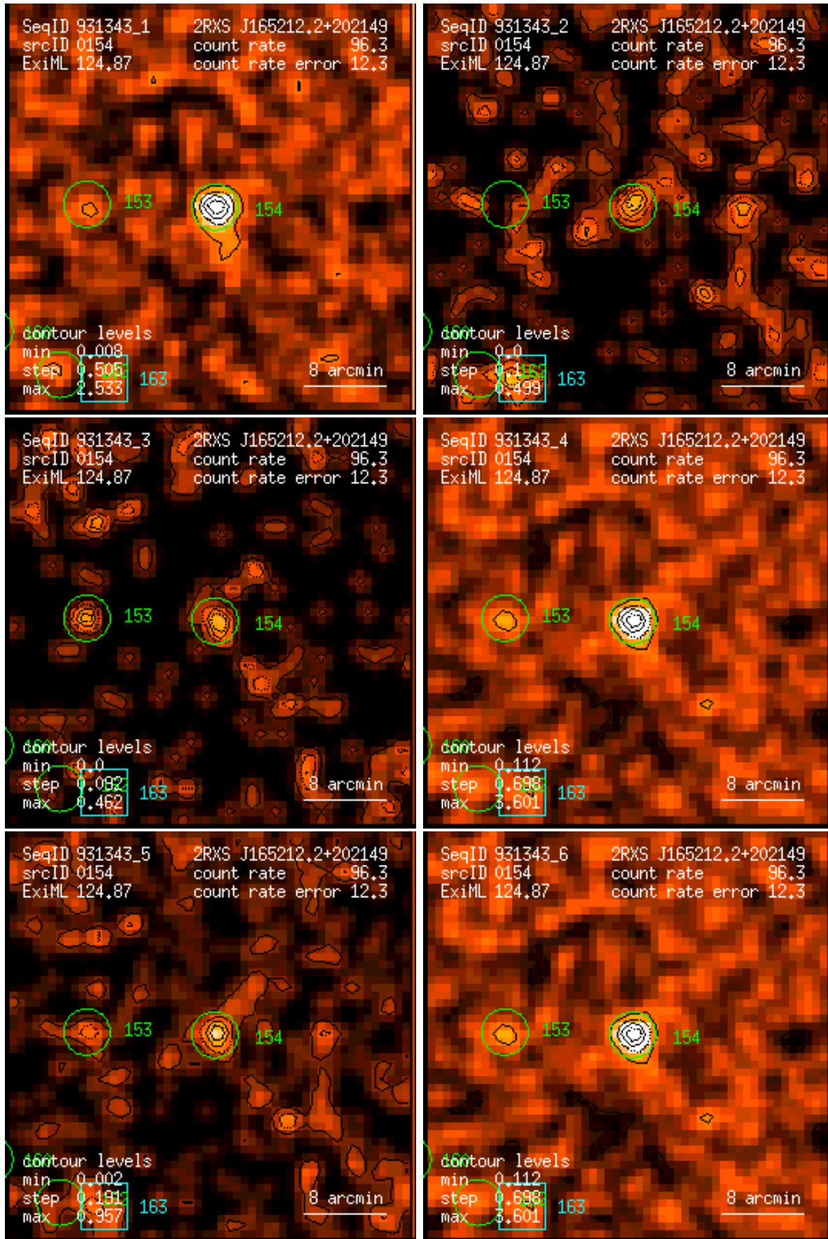
Figure 154: RASS 931343: detection 0154: band rate images, Gaussian filter: (1) PSPC channels 11 – 41, (2) 52 – 90, (3) 91 – 201, (4) 11 – 235, (5) 52 – 201, (6) 11 – 201. Broad band rates in counts/ks. Band rate contour levels in counts/ks/arcmin 2 .
