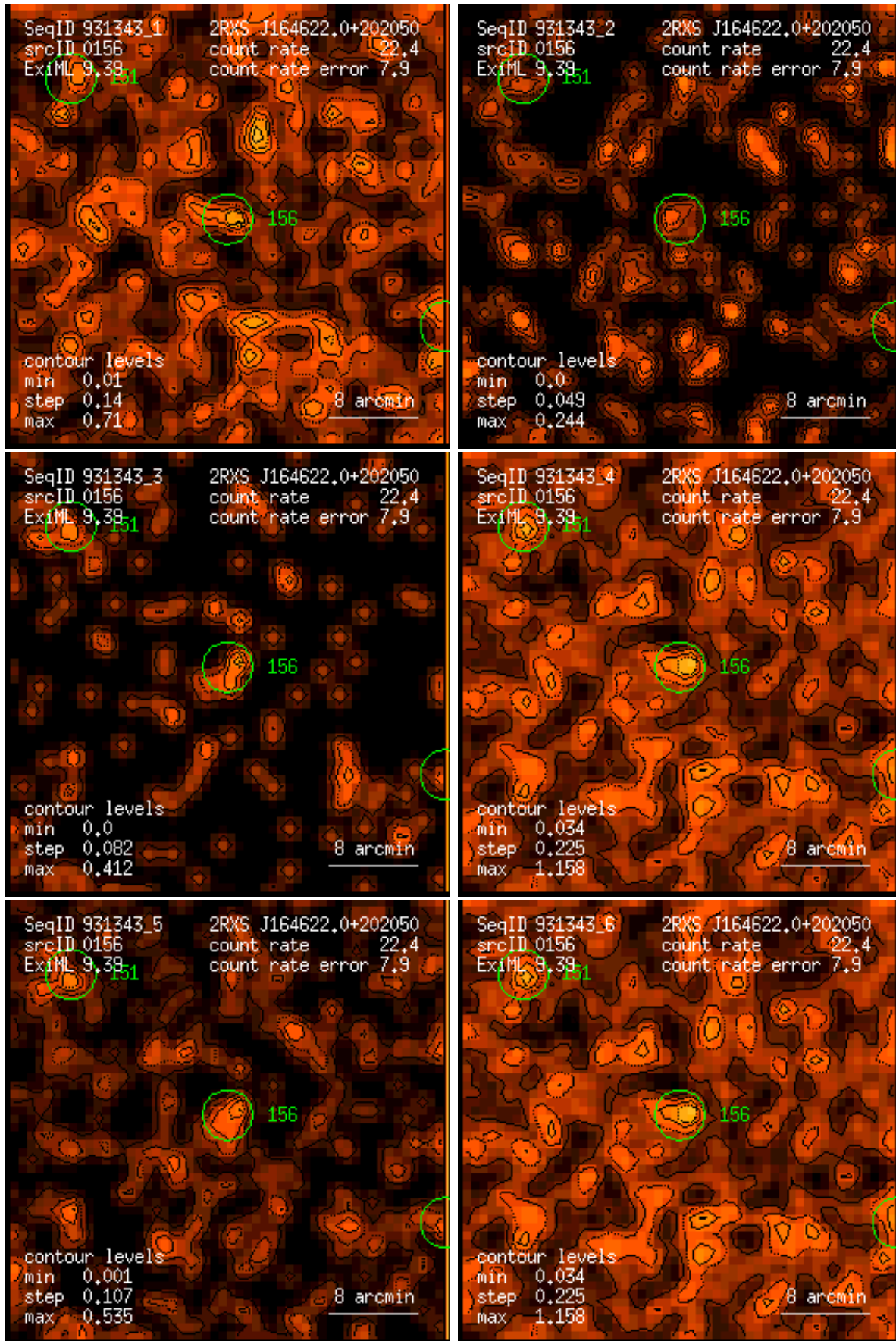
Figure 156: RASS 931343: detection 0156: band rate images, Gaussian filter: (1) PSPC channels 11 – 41, (2) 52 – 90, (3) 91 – 201, (4) 11 – 235, (5) 52 – 201, (6) 11 – 201. Broad band rates in counts/ks. Band rate contour levels in counts/ks/arcmin 2 .
