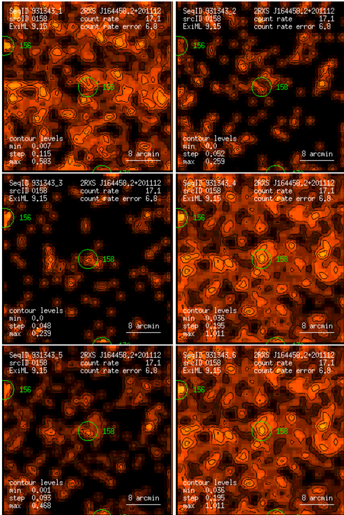
Figure 158: RASS 931343: detection 0158: band rate images, Gaussian filter: (1) PSPC channels 11 – 41, (2) 52 – 90, (3) 91 – 201, (4) 11 – 235, (5) 52 – 201, (6) 11 – 201. Broad band rates in counts/ks. Band rate contour levels in counts/ks/arcmin 2 .
