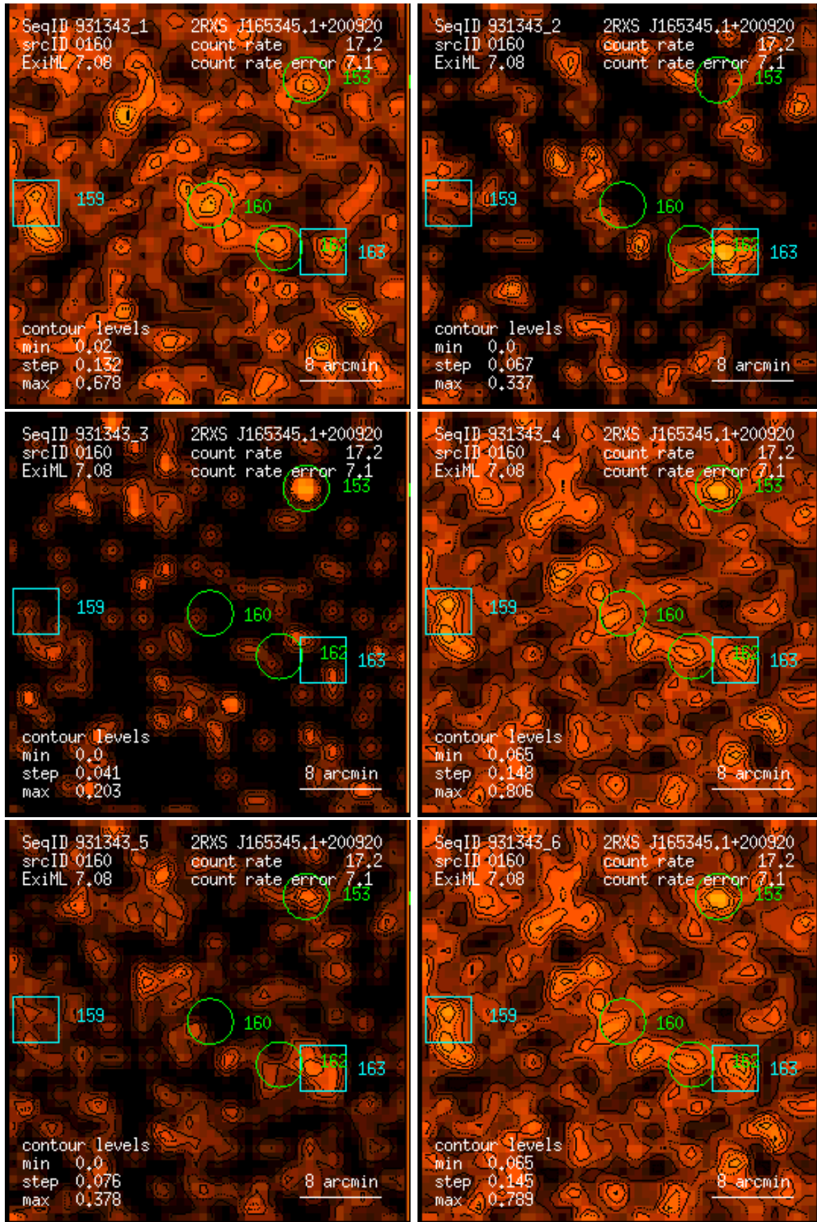
Figure 160: RASS 931343: detection 0160: band rate images, Gaussian filter: (1) PSPC channels 11 – 41, (2) 52 – 90, (3) 91 – 201, (4) 11 – 235, (5) 52 – 201, (6) 11 – 201. Broad band rates in counts/ks. Band rate contour levels in counts/ks/arcmin 2 .
