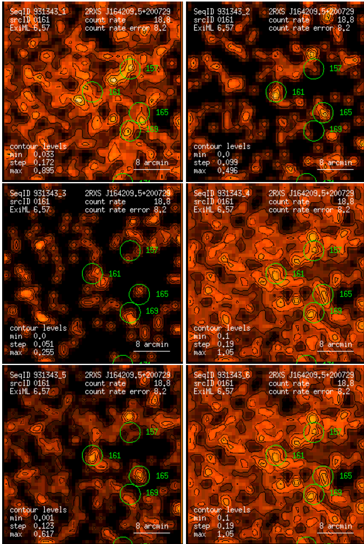
Figure 161: RASS 931343: detection 0161: band rate images, Gaussian filter: (1) PSPC channels 11 – 41, (2) 52 – 90, (3) 91 – 201, (4) 11 – 235, (5) 52 – 201, (6) 11 – 201. Broad band rates in counts/ks. Band rate contour levels in counts/ks/arcmin 2 .
