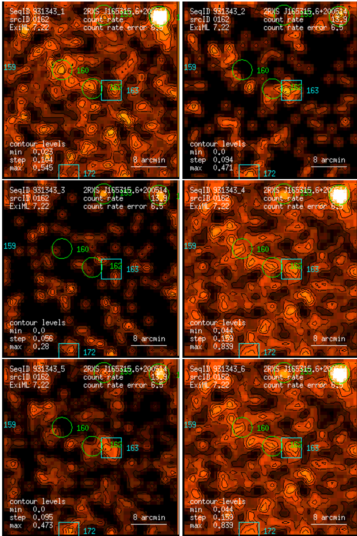
Figure 162: RASS 931343: detection 0162: band rate images, Gaussian filter: (1) PSPC channels 11 – 41, (2) 52 – 90, (3) 91 – 201, (4) 11 – 235, (5) 52 – 201, (6) 11 – 201. Broad band rates in counts/ks. Band rate contour levels in counts/ks/arcmin 2 .
