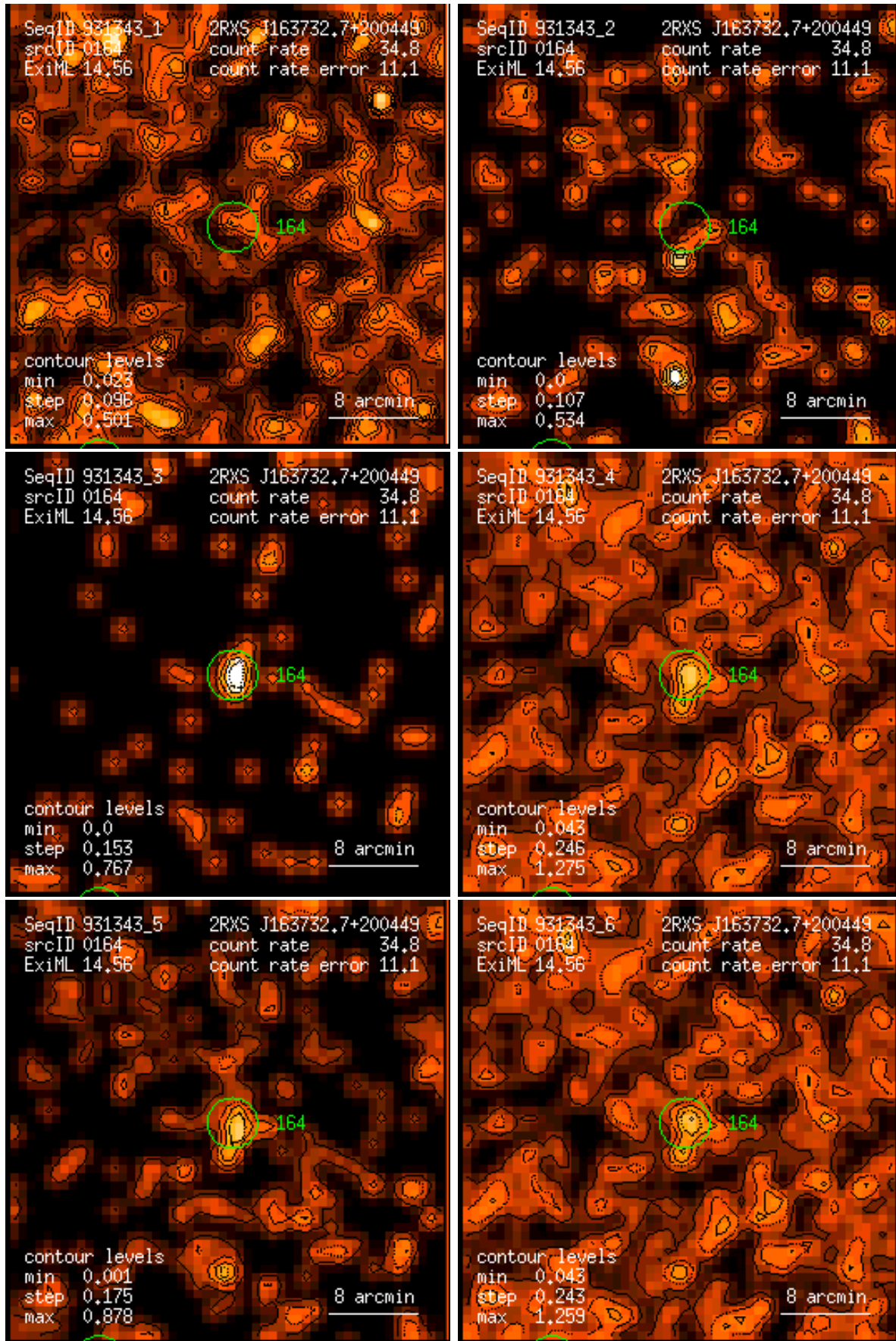
Figure 164: RASS 931343: detection 0164: band rate images, Gaussian filter: (1) PSPC channels 11 – 41, (2) 52 – 90, (3) 91 – 201, (4) 11 – 235, (5) 52 – 201, (6) 11 – 201. Broad band rates in counts/ks. Band rate contour levels in counts/ks/arcmin 2 .
