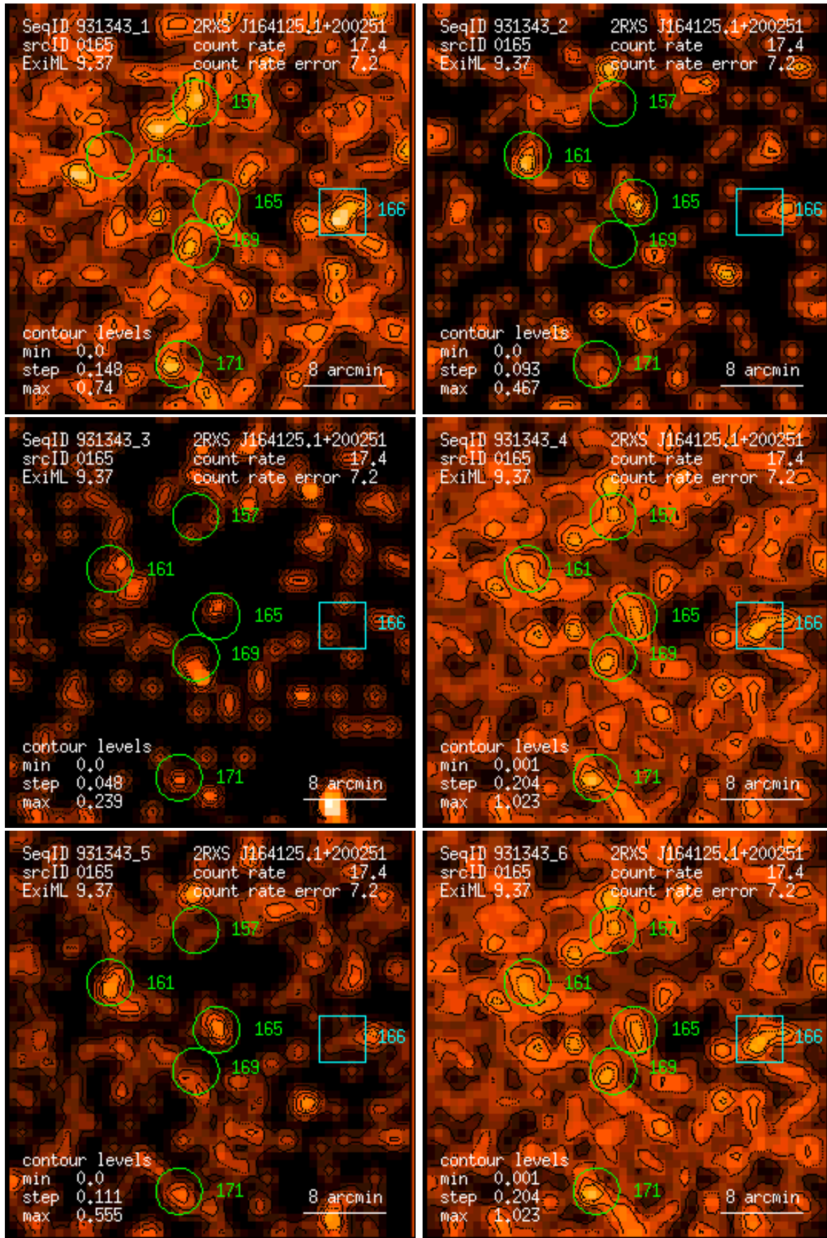
Figure 165: RASS 931343: detection 0165: band rate images, Gaussian filter: (1) PSPC channels 11 – 41, (2) 52 – 90, (3) 91 – 201, (4) 11 – 235, (5) 52 – 201, (6) 11 – 201. Broad band rates in counts/ks. Band rate contour levels in counts/ks/arcmin 2 .
