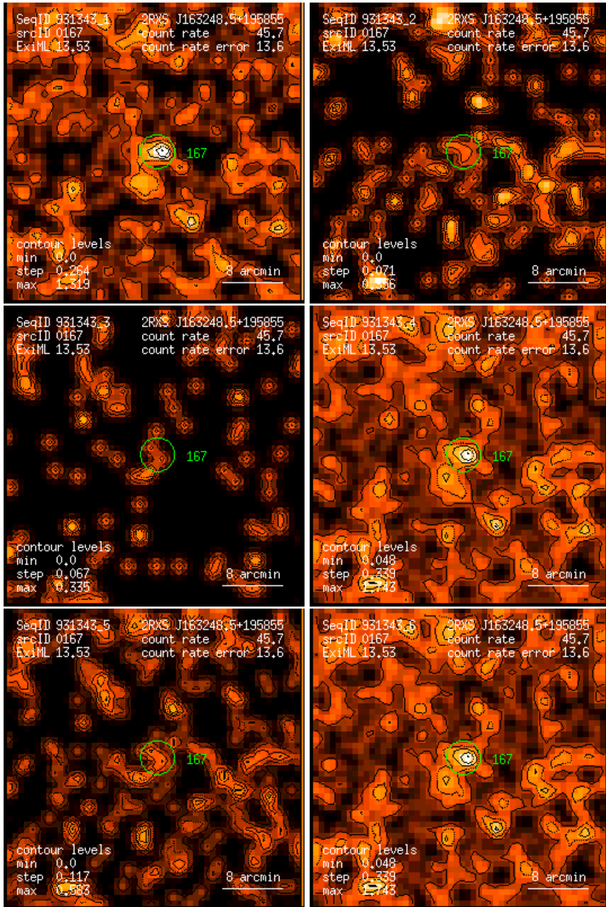
Figure 167: RASS 931343: detection 0167: band rate images, Gaussian filter: (1) PSPC channels 11 – 41, (2) 52 – 90, (3) 91 – 201, (4) 11 – 235, (5) 52 – 201, (6) 11 – 201. Broad band rates in counts/ks. Band rate contour levels in counts/ks/arcmin 2 .
