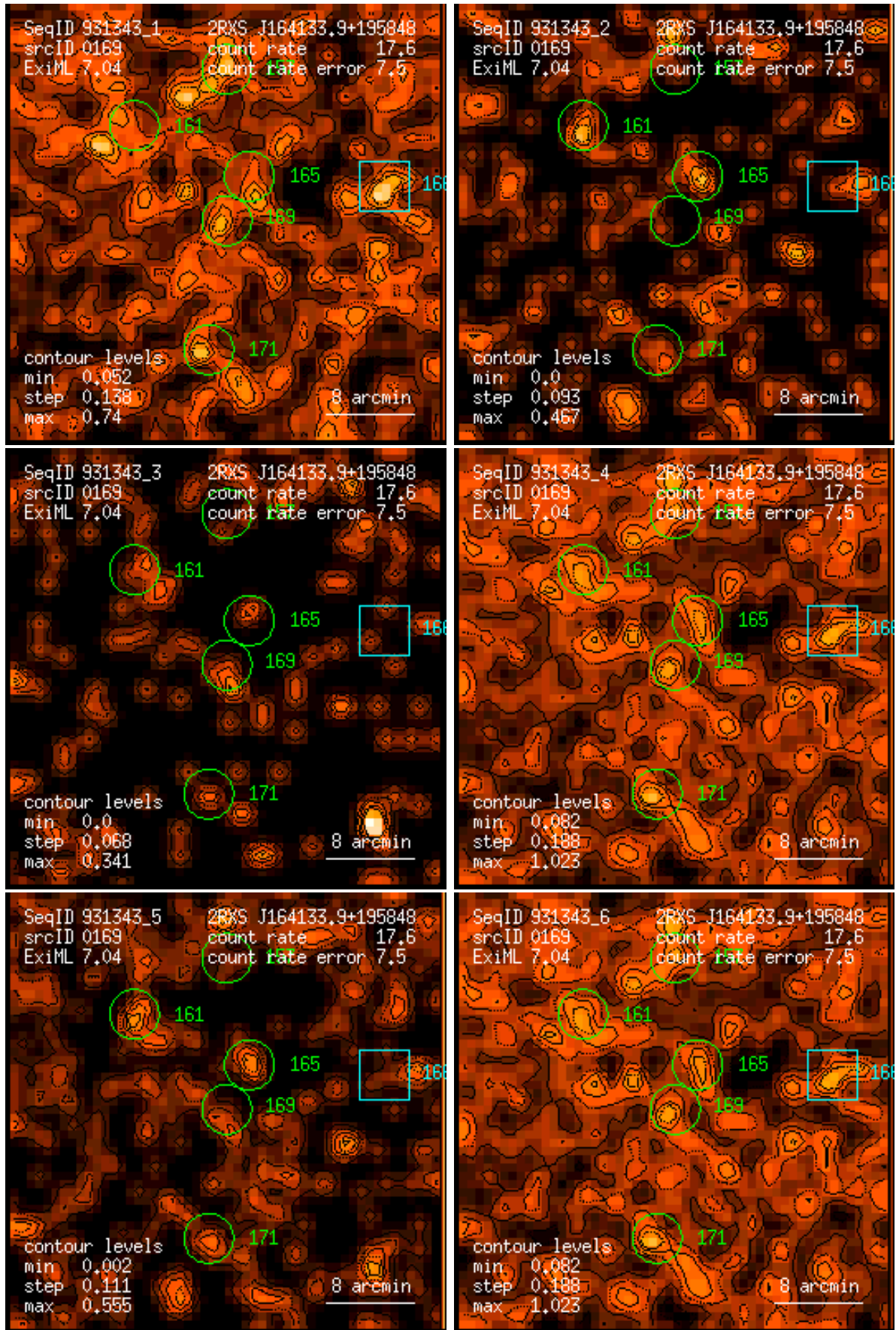
Figure 169: RASS 931343: detection 0169: band rate images, Gaussian filter: (1) PSPC channels 11 – 41, (2) 52 – 90, (3) 91 – 201, (4) 11 – 235, (5) 52 – 201, (6) 11 – 201. Broad band rates in counts/ks. Band rate contour levels in counts/ks/arcmin 2 .
