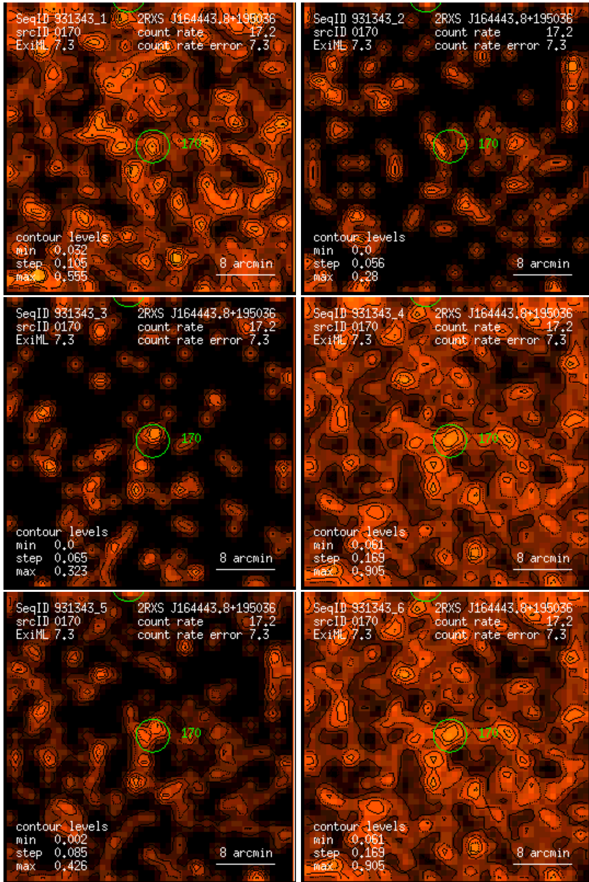
Figure 170: RASS 931343: detection 0170: band rate images, Gaussian filter: (1) PSPC channels 11 – 41, (2) 52 – 90, (3) 91 – 201, (4) 11 – 235, (5) 52 – 201, (6) 11 – 201. Broad band rates in counts/ks. Band rate contour levels in counts/ks/arcmin 2 .
