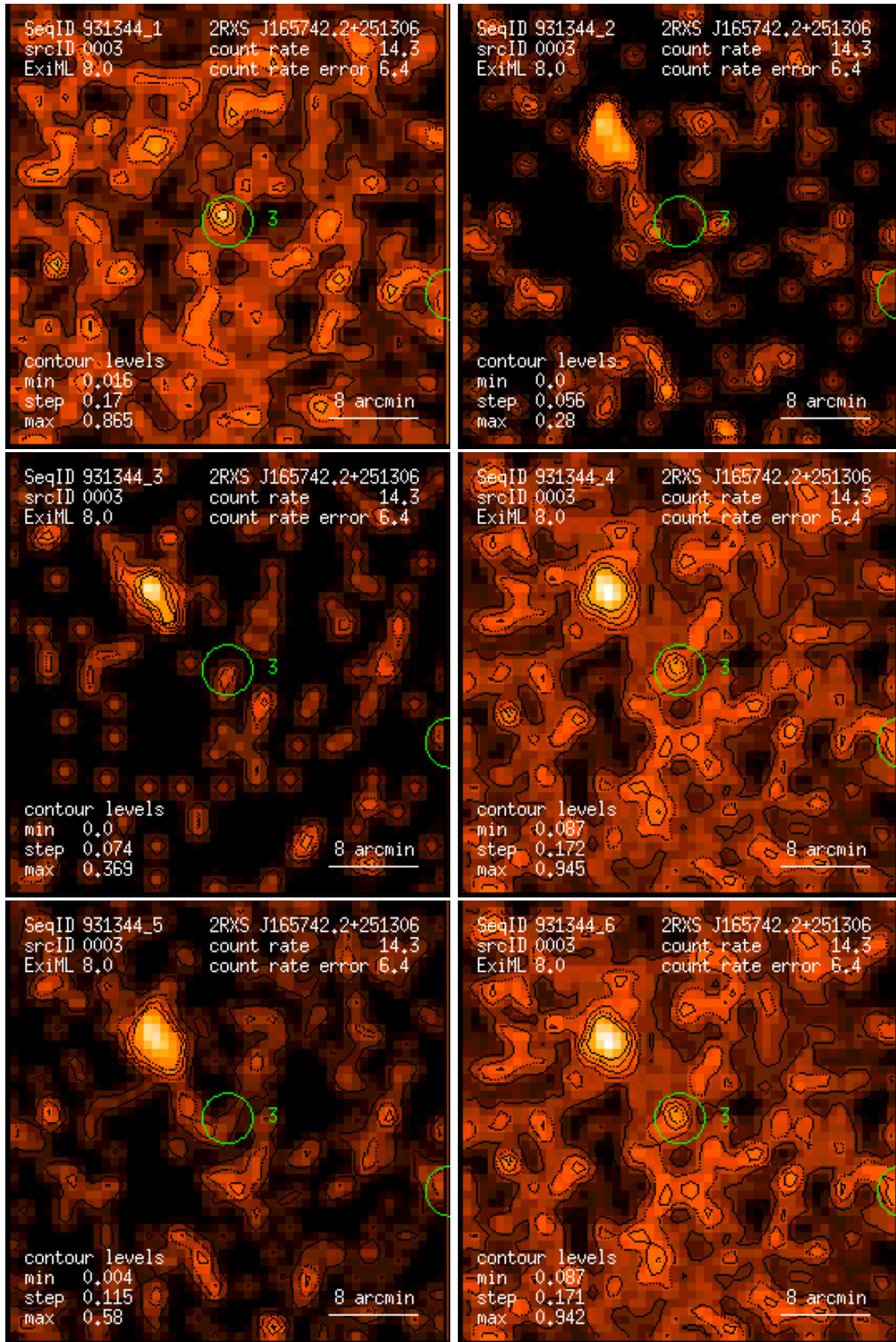
Figure 3: RASS 931344: detection 0003: band rate images, Gaussian filter: (1) PSPC channels 11 – 41, (2) 52 – 90, (3) 91 – 201, (4) 11 – 235, (5) 52 – 201, (6) 11 – 201. Broad band rates in counts/ks. Band rate contour levels in counts/ks/arcmin 2 .
