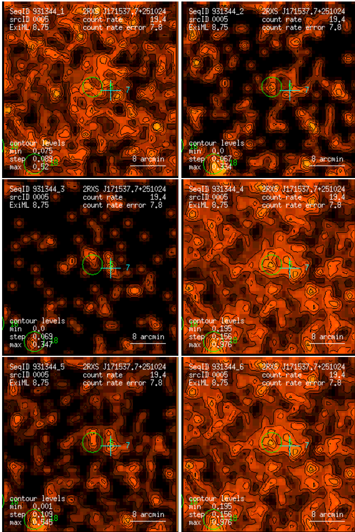
Figure 5: RASS 931344: detection 0005: band rate images, Gaussian filter: (1) PSPC channels 11 – 41, (2) 52 – 90, (3) 91 – 201, (4) 11 – 235, (5) 52 – 201, (6) 11 – 201. Broad band rates in counts/ks. Band rate contour levels in counts/ks/arcmin 2 .
