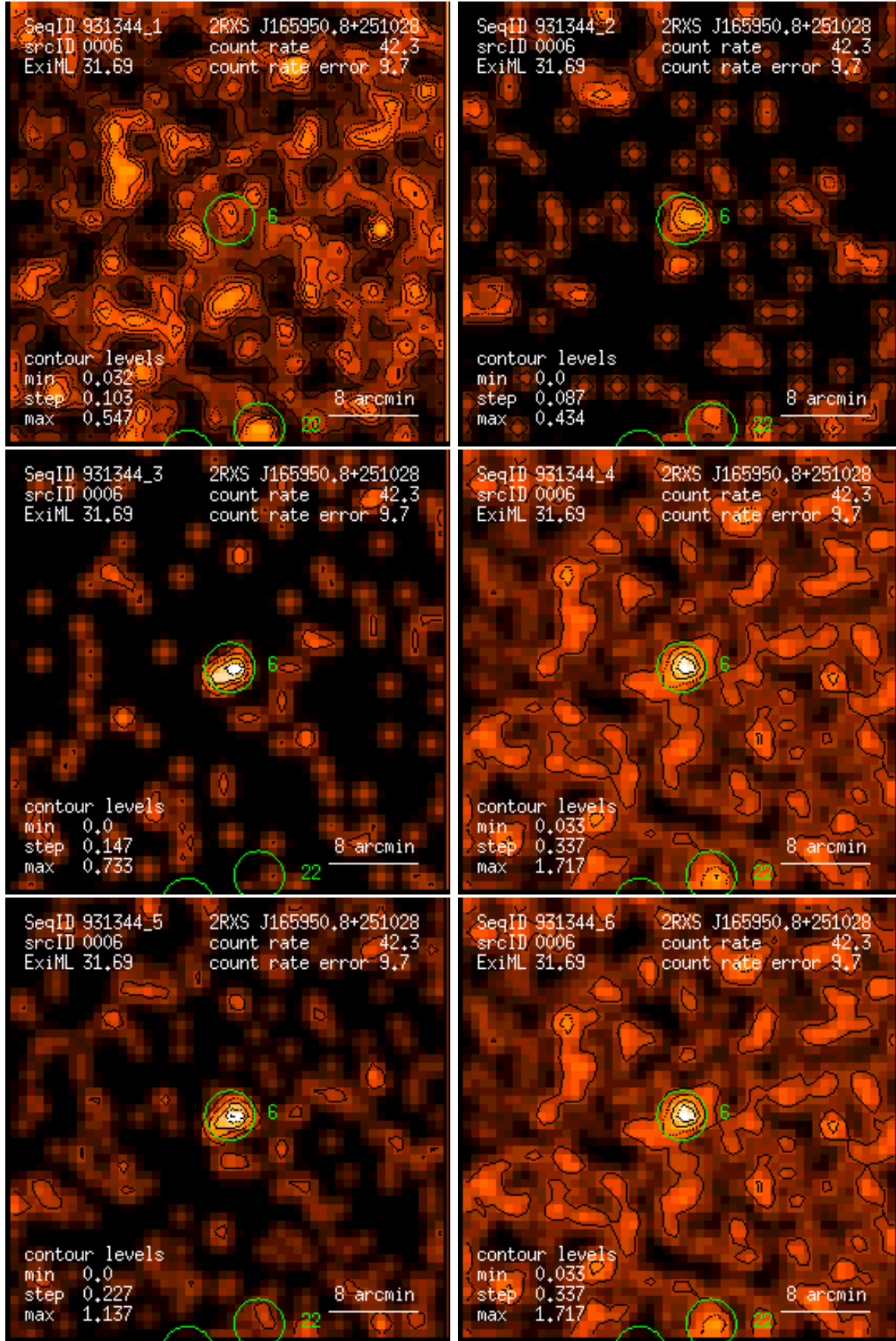
Figure 6: RASS 931344: detection 0006: band rate images, Gaussian filter: (1) PSPC channels 11 – 41, (2) 52 – 90, (3) 91 – 201, (4) 11 – 235, (5) 52 – 201, (6) 11 – 201. Broad band rates in counts/ks. Band rate contour levels in counts/ks/arcmin 2 .
