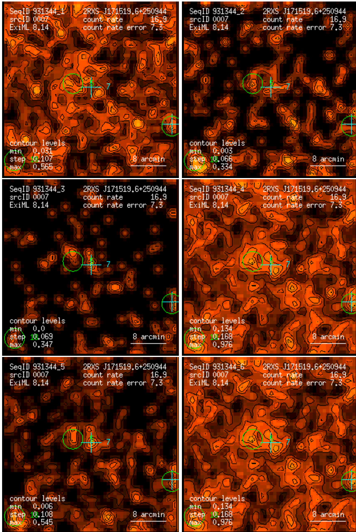
Figure 7: RASS 931344: detection 0007: band rate images, Gaussian filter: (1) PSPC channels 11 – 41, (2) 52 – 90, (3) 91 – 201, (4) 11 – 235, (5) 52 – 201, (6) 11 – 201. Broad band rates in counts/ks. Band rate contour levels in counts/ks/arcmin 2 .
