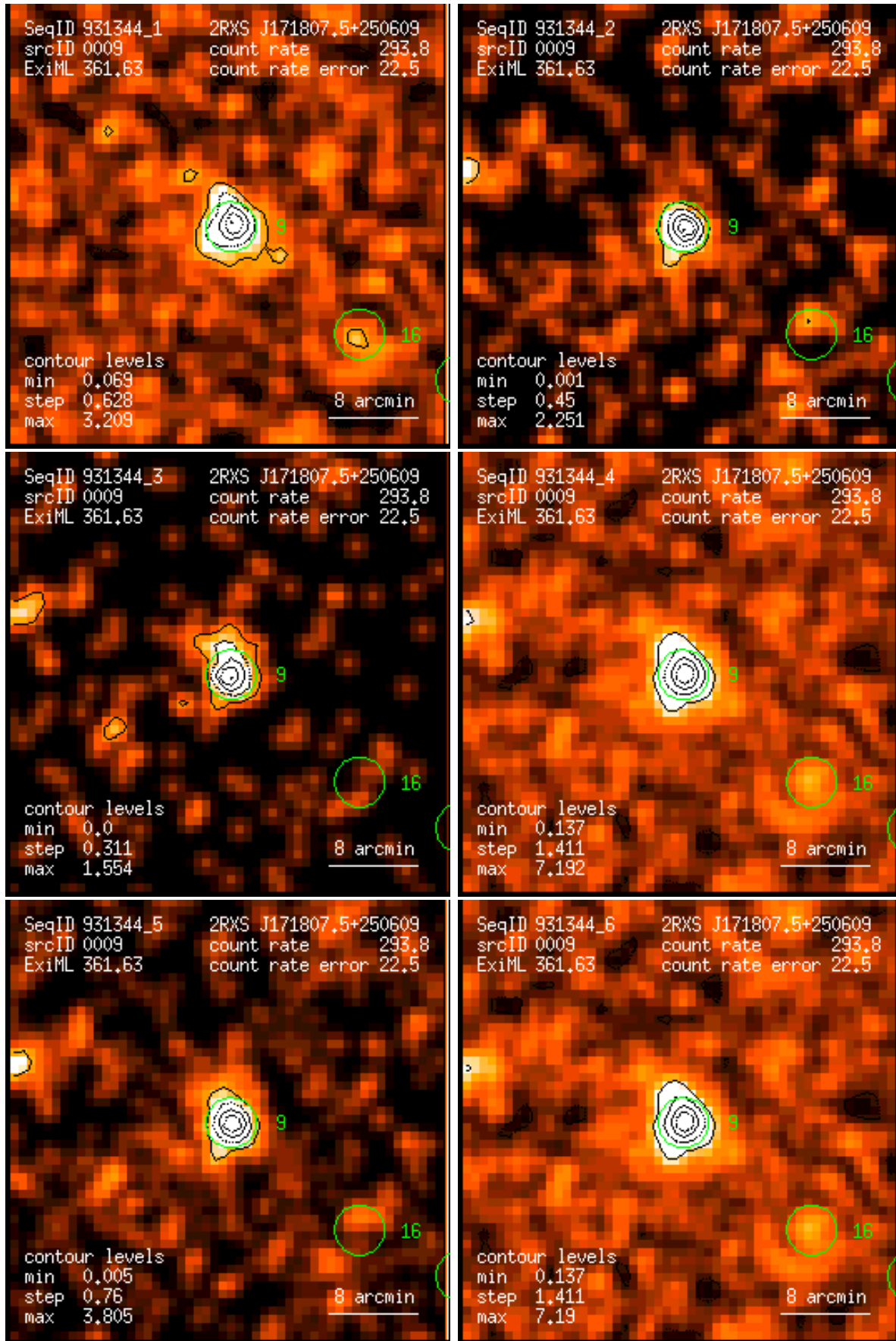
Figure 9: RASS 931344: detection 0009: band rate images, Gaussian filter: (1) PSPC channels 11 – 41, (2) 52 – 90, (3) 91 – 201, (4) 11 – 235, (5) 52 – 201, (6) 11 – 201. Broad band rates in counts/ks. Band rate contour levels in counts/ks/arcmin 2 .
