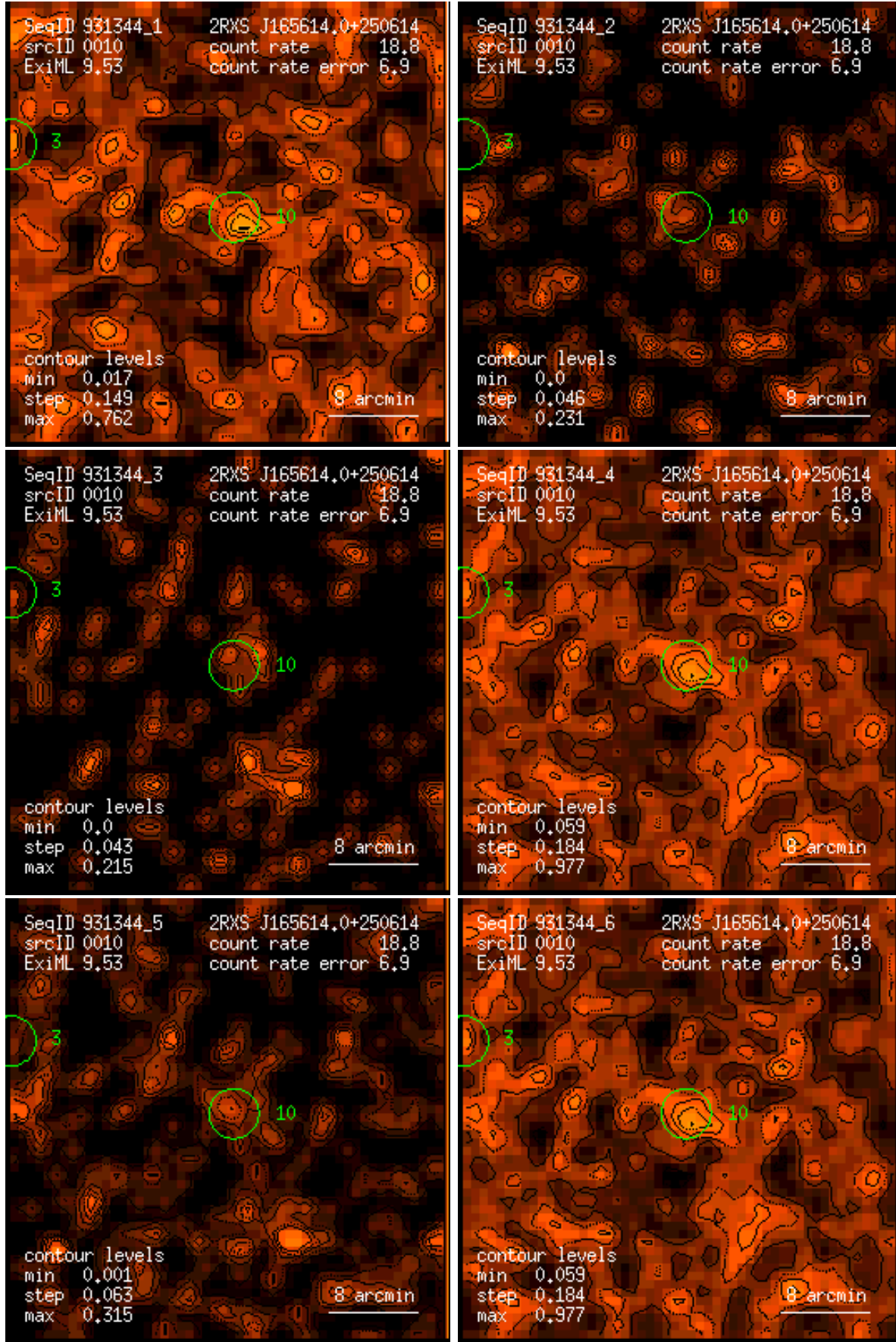
Figure 10: RASS 931344: detection 0010: band rate images, Gaussian filter: (1) PSPC channels 11 – 41, (2) 52 – 90, (3) 91 – 201, (4) 11 – 235, (5) 52 – 201, (6) 11 – 201. Broad band rates in counts/ks. Band rate contour levels in counts/ks/arcmin 2 .
