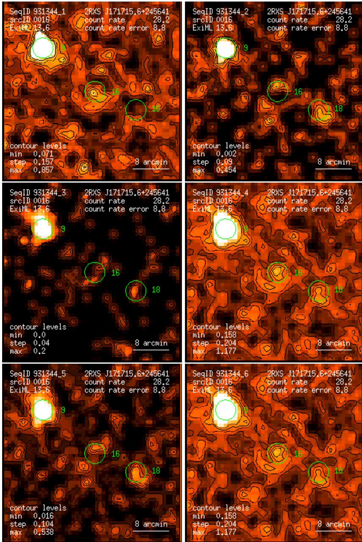
Figure 16: RASS 931344: detection 0016: band rate images, Gaussian filter: (1) PSPC channels 11 – 41, (2) 52 – 90, (3) 91 – 201, (4) 11 – 235, (5) 52 – 201, (6) 11 – 201. Broad band rates in counts/ks. Band rate contour levels in counts/ks/arcmin 2 .
