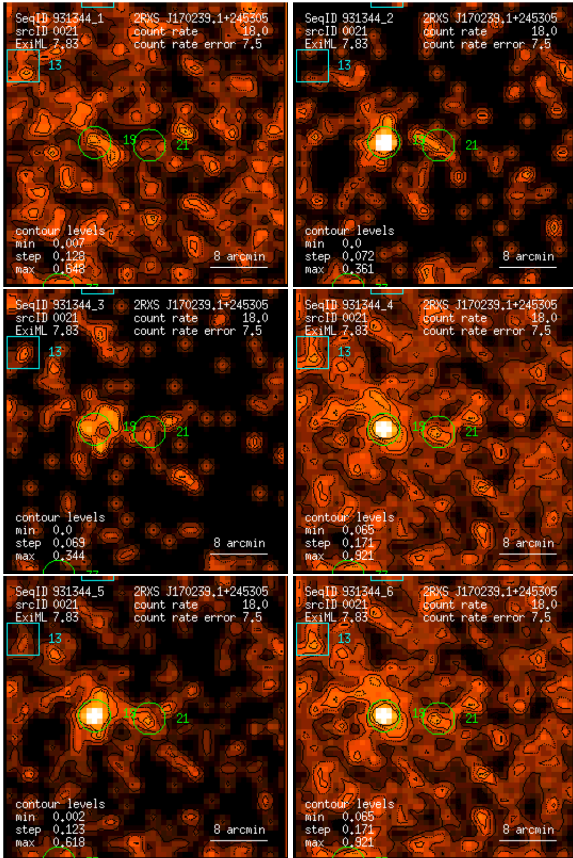
Figure 21: RASS 931344: detection 0021: band rate images, Gaussian filter: (1) PSPC channels 11 – 41, (2) 52 – 90, (3) 91 – 201, (4) 11 – 235, (5) 52 – 201, (6) 11 – 201. Broad band rates in counts/ks. Band rate contour levels in counts/ks/arcmin 2 .
