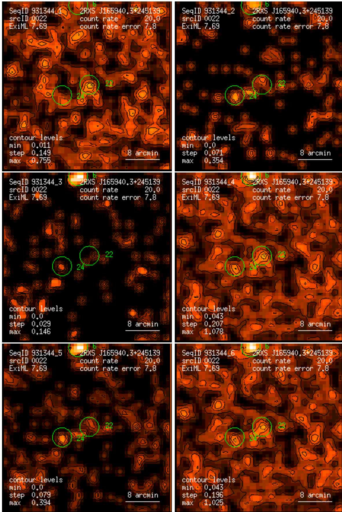
Figure 22: RASS 931344: detection 0022: band rate images, Gaussian filter: (1) PSPC channels 11 – 41, (2) 52 – 90, (3) 91 – 201, (4) 11 – 235, (5) 52 – 201, (6) 11 – 201. Broad band rates in counts/ks. Band rate contour levels in counts/ks/arcmin 2 .
