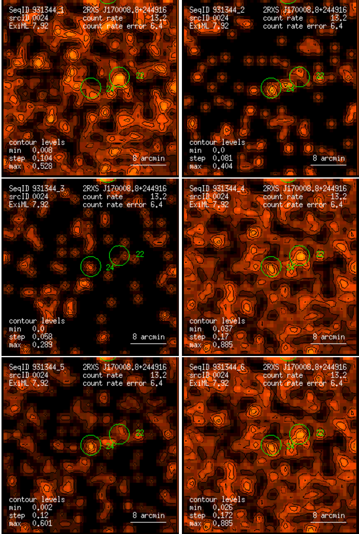
Figure 24: RASS 931344: detection 0024: band rate images, Gaussian filter: (1) PSPC channels 11 – 41, (2) 52 – 90, (3) 91 – 201, (4) 11 – 235, (5) 52 – 201, (6) 11 – 201. Broad band rates in counts/ks. Band rate contour levels in counts/ks/arcmin 2 .
