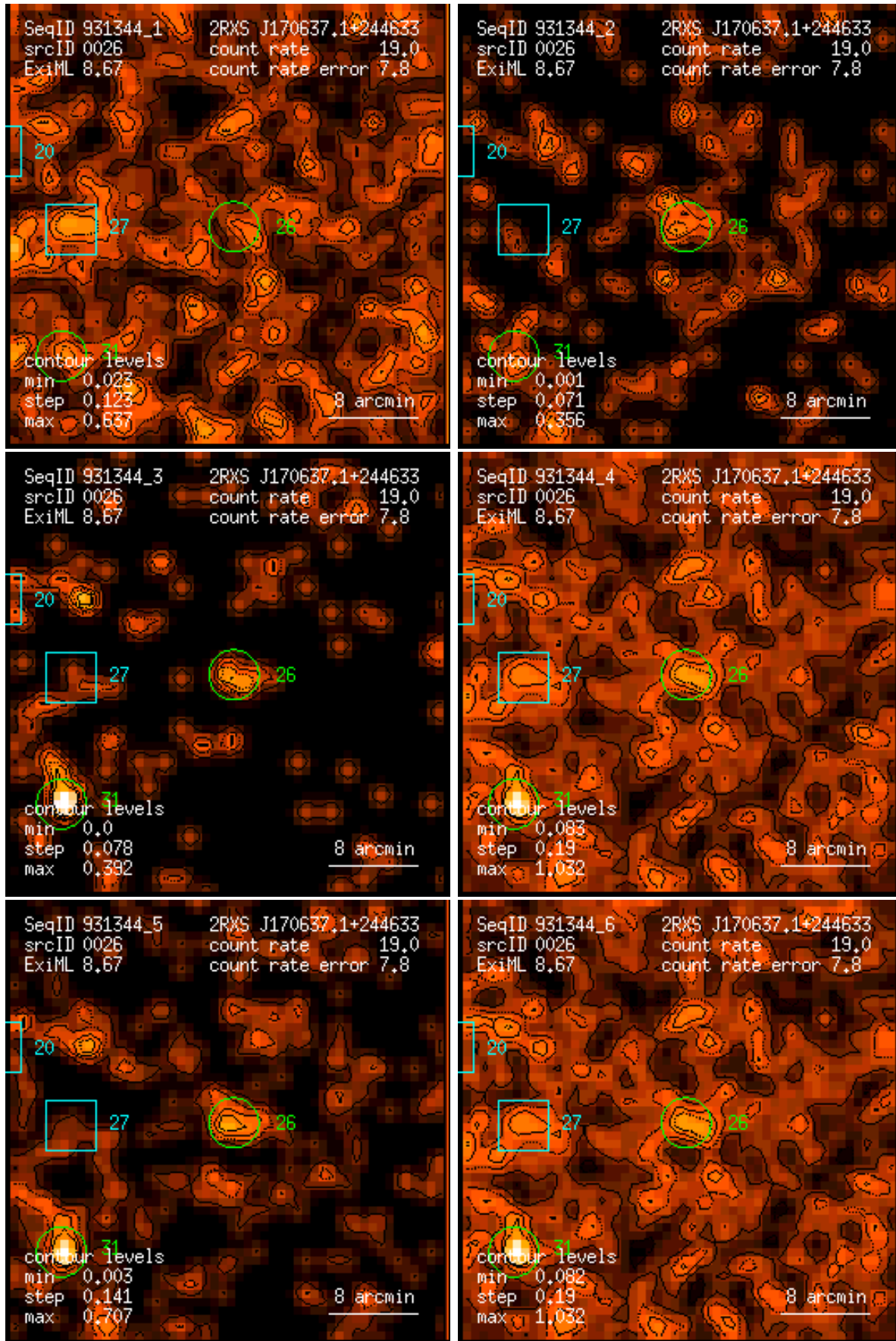
Figure 26: RASS 931344: detection 0026: band rate images, Gaussian filter: (1) PSPC channels 11 – 41, (2) 52 – 90, (3) 91 – 201, (4) 11 – 235, (5) 52 – 201, (6) 11 – 201. Broad band rates in counts/ks. Band rate contour levels in counts/ks/arcmin 2 .
