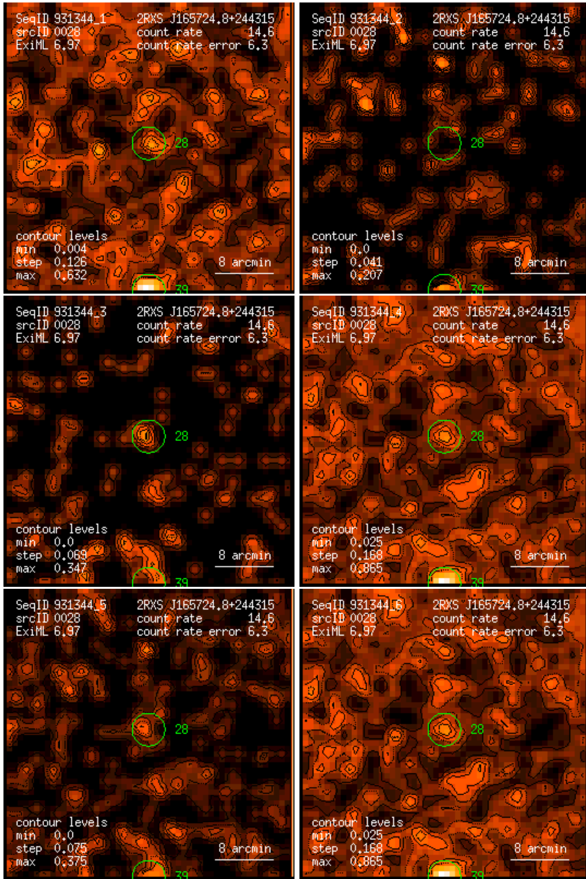
Figure 28: RASS 931344: detection 0028: band rate images, Gaussian filter: (1) PSPC channels 11 – 41, (2) 52 – 90, (3) 91 – 201, (4) 11 – 235, (5) 52 – 201, (6) 11 – 201. Broad band rates in counts/ks. Band rate contour levels in counts/ks/arcmin 2 .
