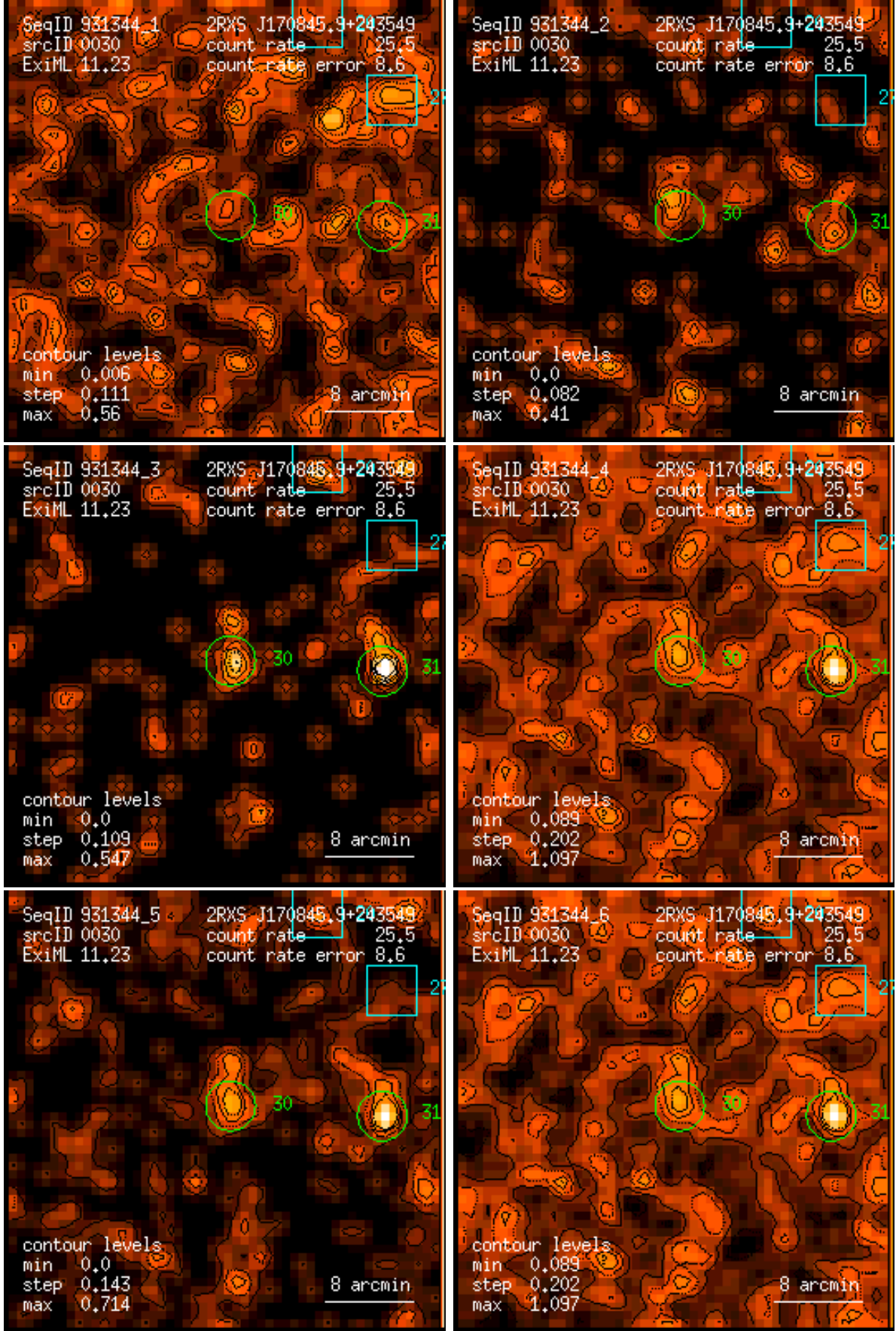
Figure 30: RASS 931344: detection 0030: band rate images, Gaussian filter: (1) PSPC channels 11 – 41, (2) 52 – 90, (3) 91 – 201, (4) 11 – 235, (5) 52 – 201, (6) 11 – 201. Broad band rates in counts/ks. Band rate contour levels in counts/ks/arcmin 2 .
