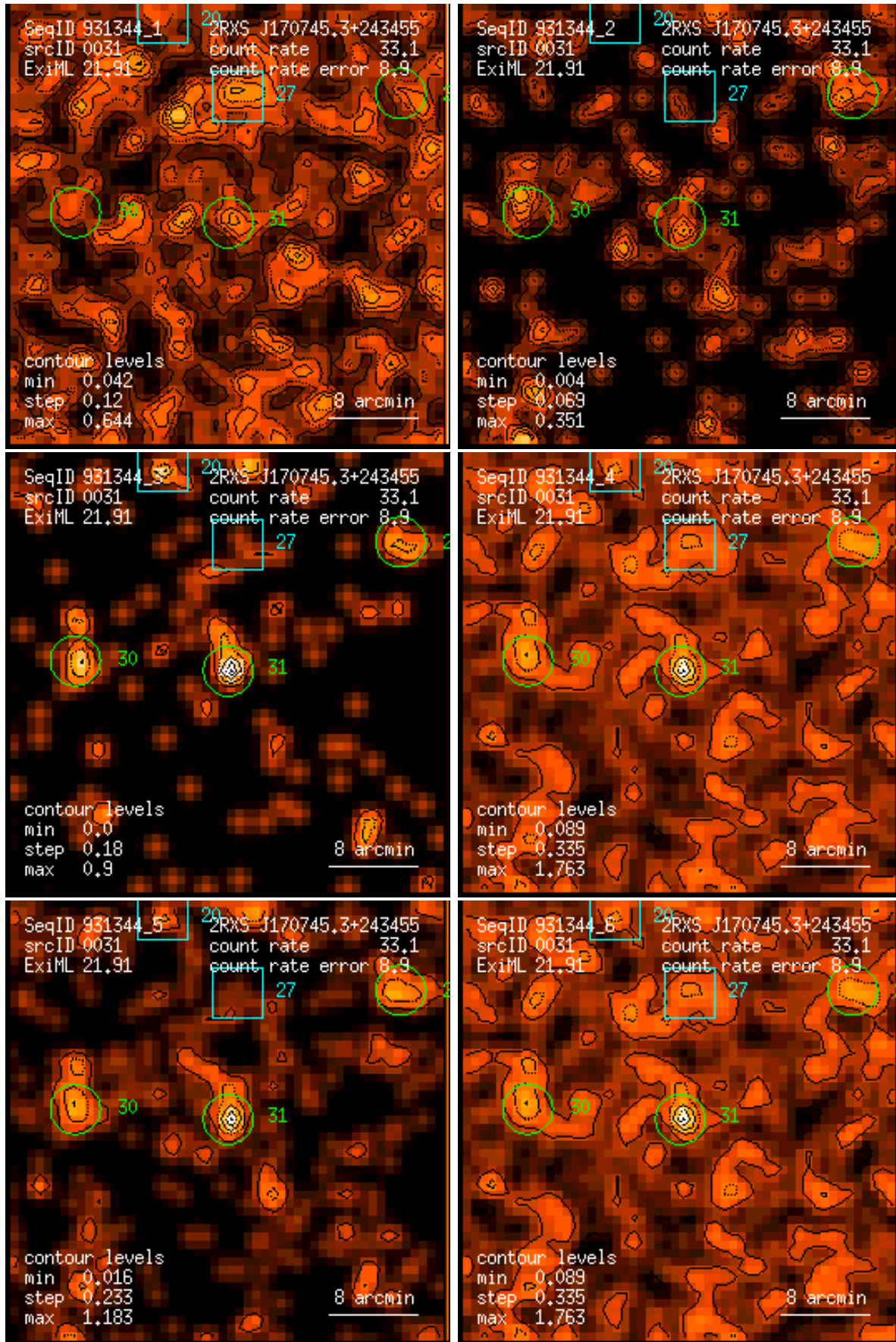
Figure 31: RASS 931344: detection 0031: band rate images, Gaussian filter: (1) PSPC channels 11 – 41, (2) 52 – 90, (3) 91 – 201, (4) 11 – 235, (5) 52 – 201, (6) 11 – 201. Broad band rates in counts/ks. Band rate contour levels in counts/ks/arcmin 2 .
