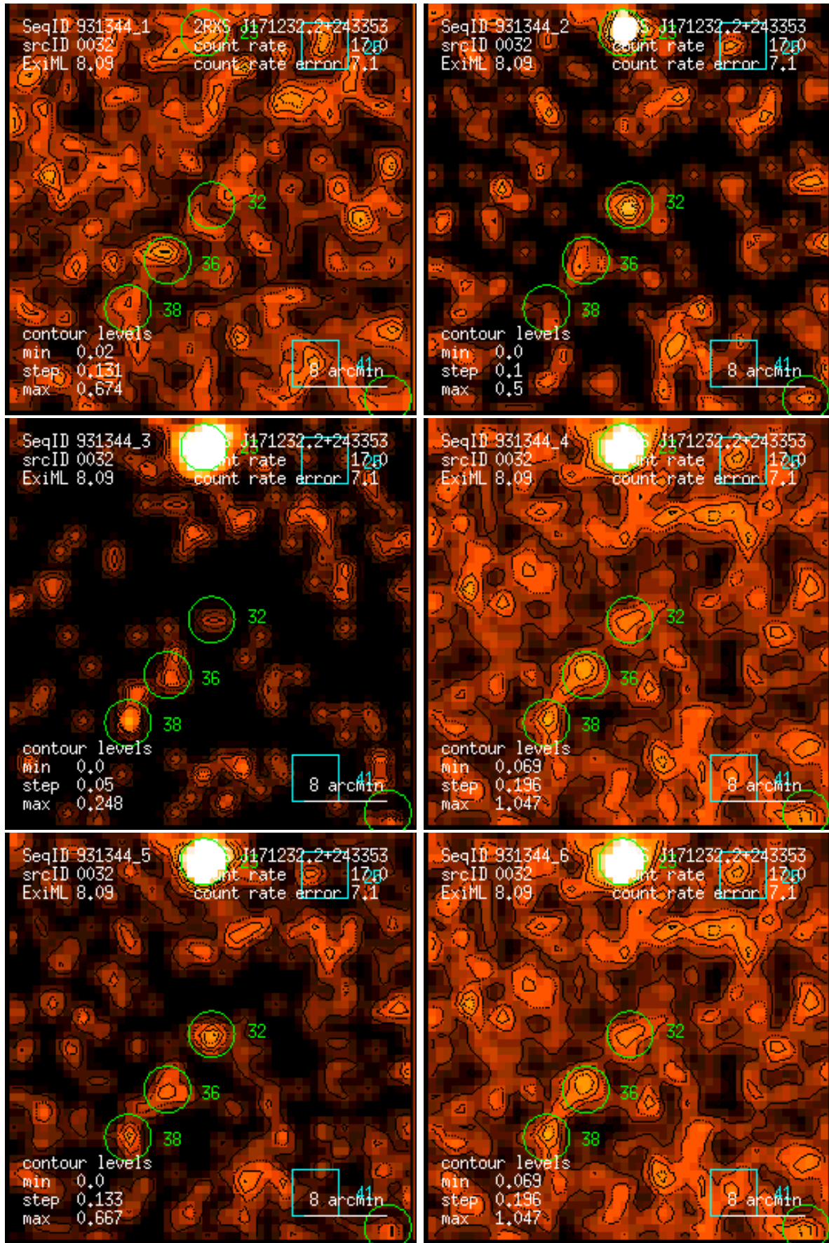
Figure 32: RASS 931344: detection 0032: band rate images, Gaussian filter: (1) PSPC channels 11 – 41, (2) 52 – 90, (3) 91 – 201, (4) 11 – 235, (5) 52 – 201, (6) 11 – 201. Broad band rates in counts/ks. Band rate contour levels in counts/ks/arcmin 2 .
