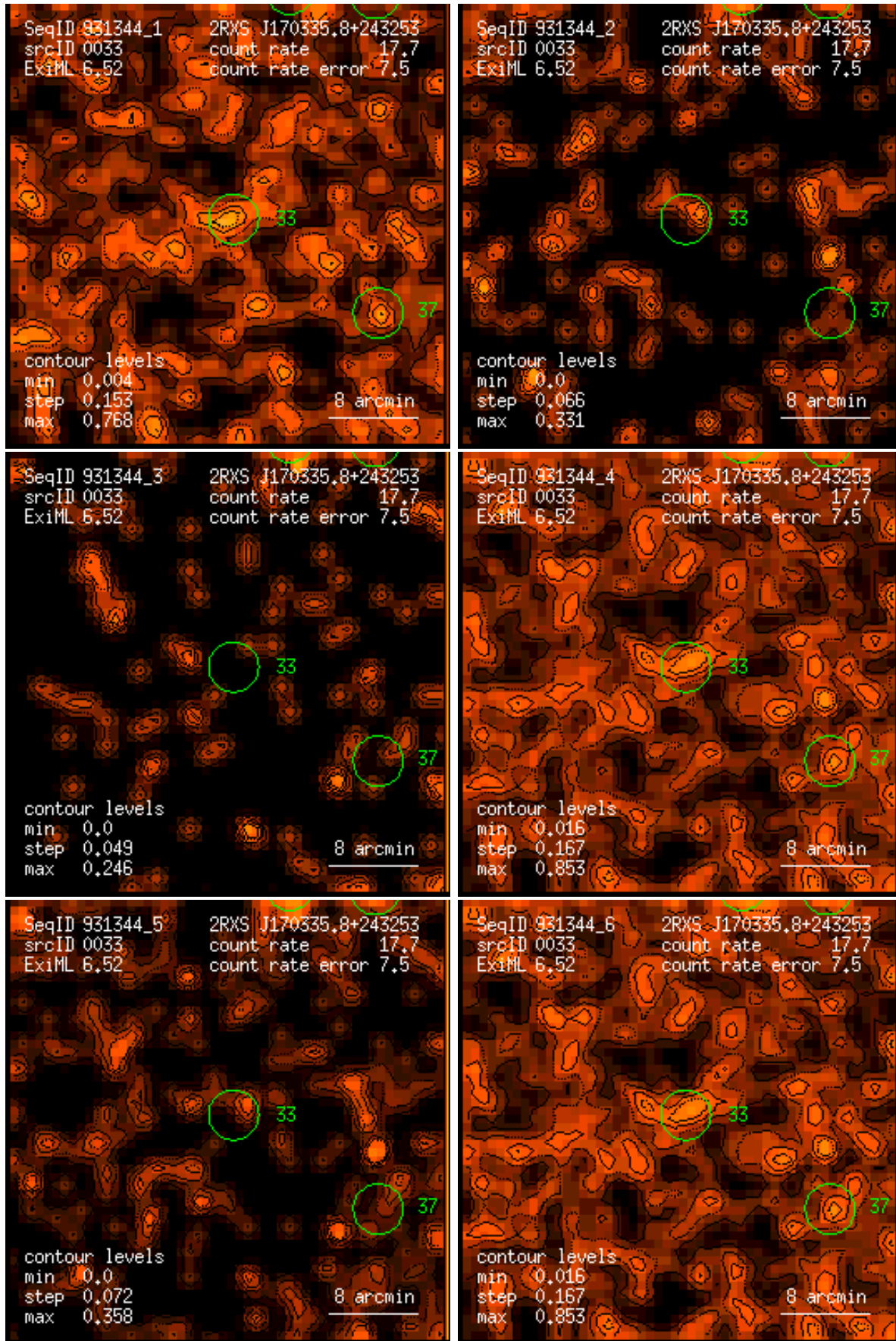
Figure 33: RASS 931344: detection 0033: band rate images, Gaussian filter: (1) PSPC channels 11 – 41, (2) 52 – 90, (3) 91 – 201, (4) 11 – 235, (5) 52 – 201, (6) 11 – 201. Broad band rates in counts/ks. Band rate contour levels in counts/ks/arcmin 2 .
