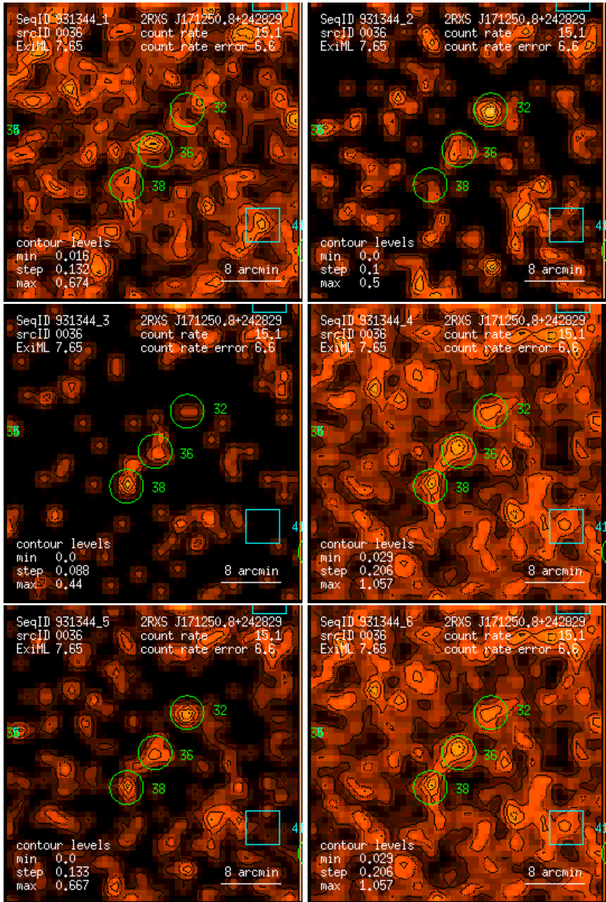
Figure 36: RASS 931344: detection 0036: band rate images, Gaussian filter: (1) PSPC channels 11 – 41, (2) 52 – 90, (3) 91 – 201, (4) 11 – 235, (5) 52 – 201, (6) 11 – 201. Broad band rates in counts/ks. Band rate contour levels in counts/ks/arcmin 2 .
