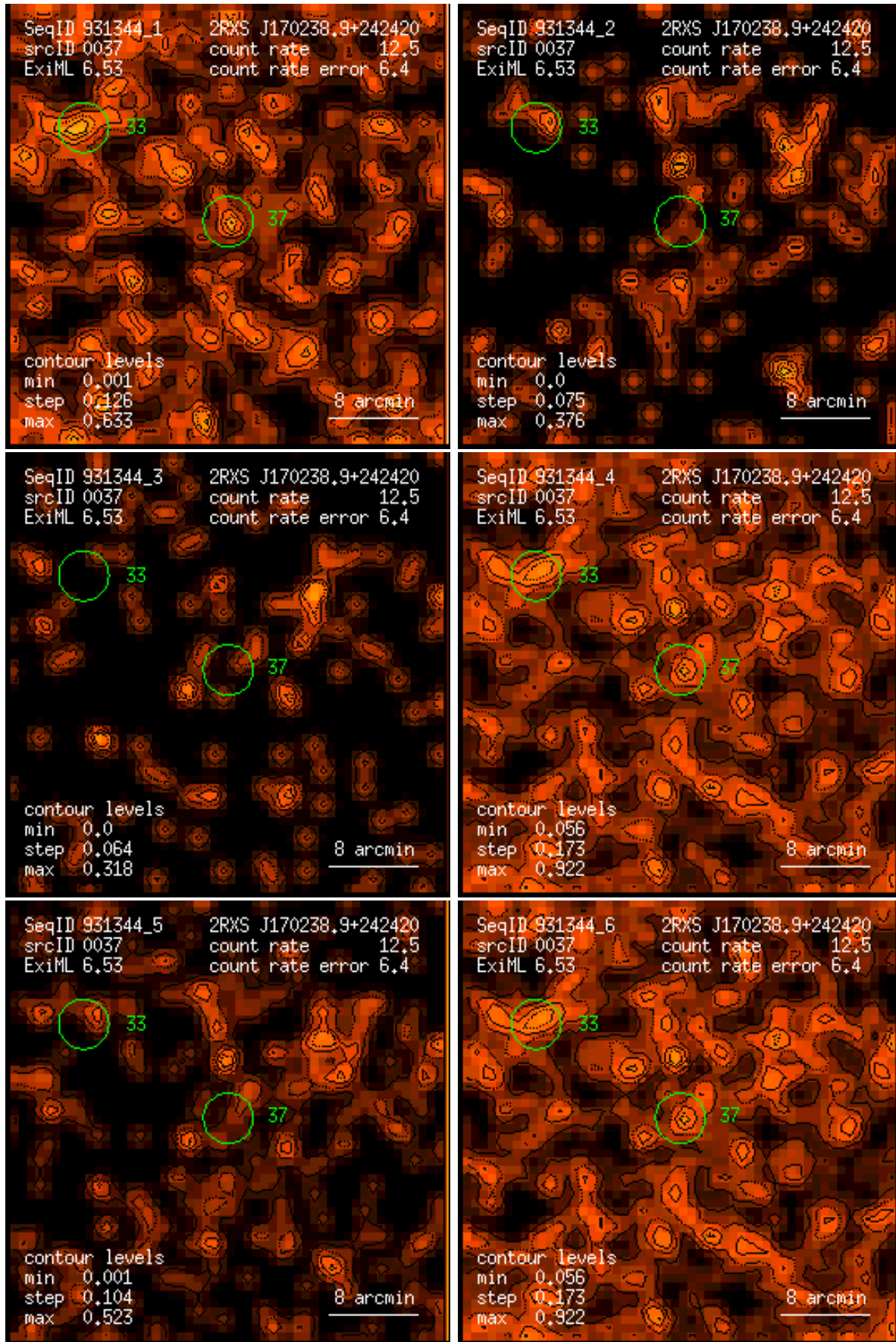
Figure 37: RASS 931344: detection 0037: band rate images, Gaussian filter: (1) PSPC channels 11 – 41, (2) 52 – 90, (3) 91 – 201, (4) 11 – 235, (5) 52 – 201, (6) 11 – 201. Broad band rates in counts/ks. Band rate contour levels in counts/ks/arcmin 2 .
