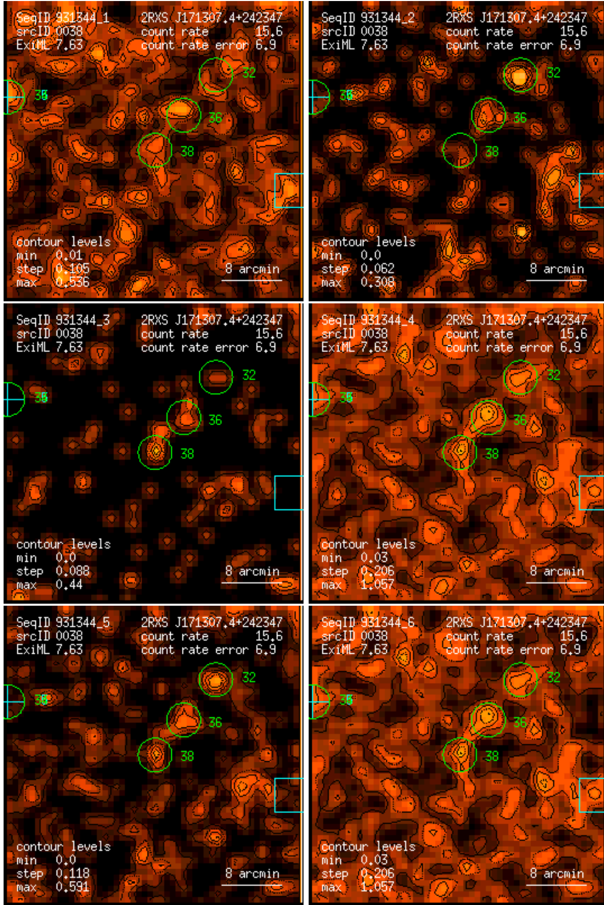
Figure 38: RASS 931344: detection 0038: band rate images, Gaussian filter: (1) PSPC channels 11 – 41, (2) 52 – 90, (3) 91 – 201, (4) 11 – 235, (5) 52 – 201, (6) 11 – 201. Broad band rates in counts/ks. Band rate contour levels in counts/ks/arcmin 2 .
