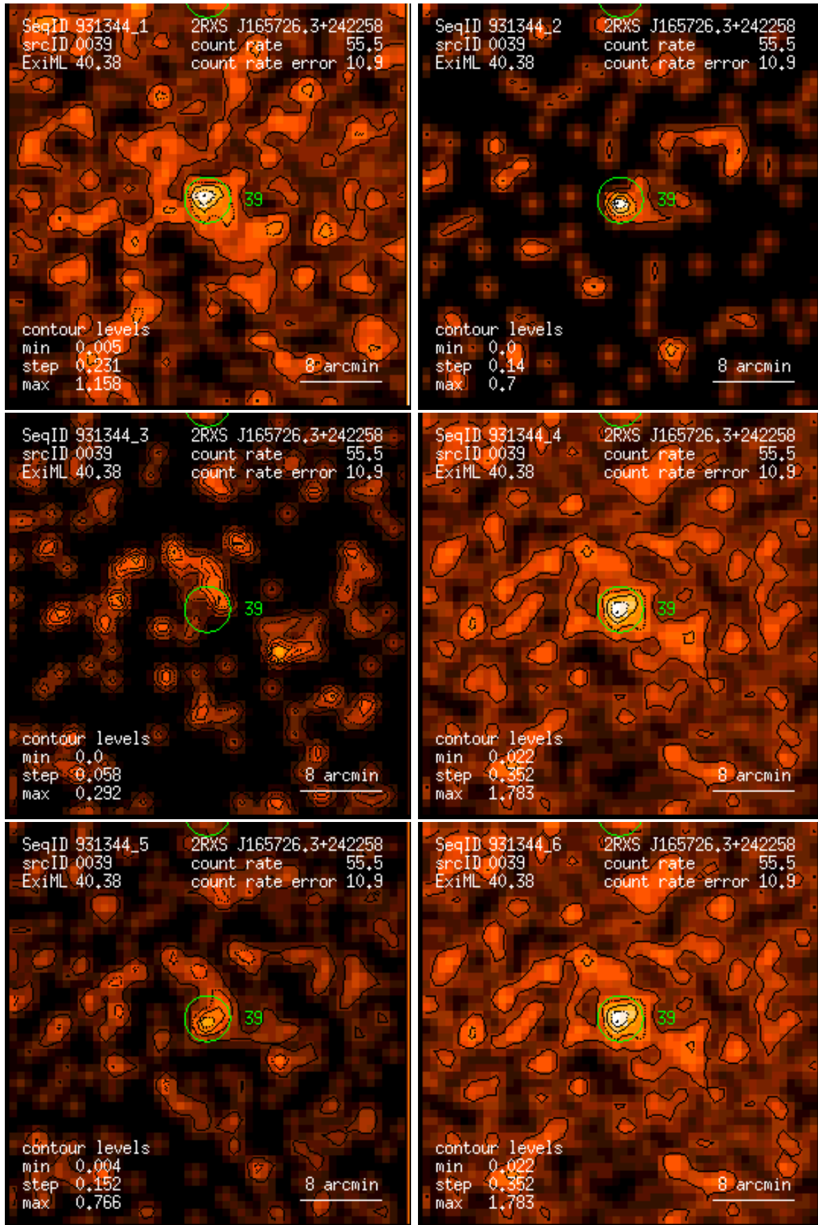
Figure 39: RASS 931344: detection 0039: band rate images, Gaussian filter: (1) PSPC channels 11 – 41, (2) 52 – 90, (3) 91 – 201, (4) 11 – 235, (5) 52 – 201, (6) 11 – 201. Broad band rates in counts/ks. Band rate contour levels in counts/ks/arcmin 2 .
