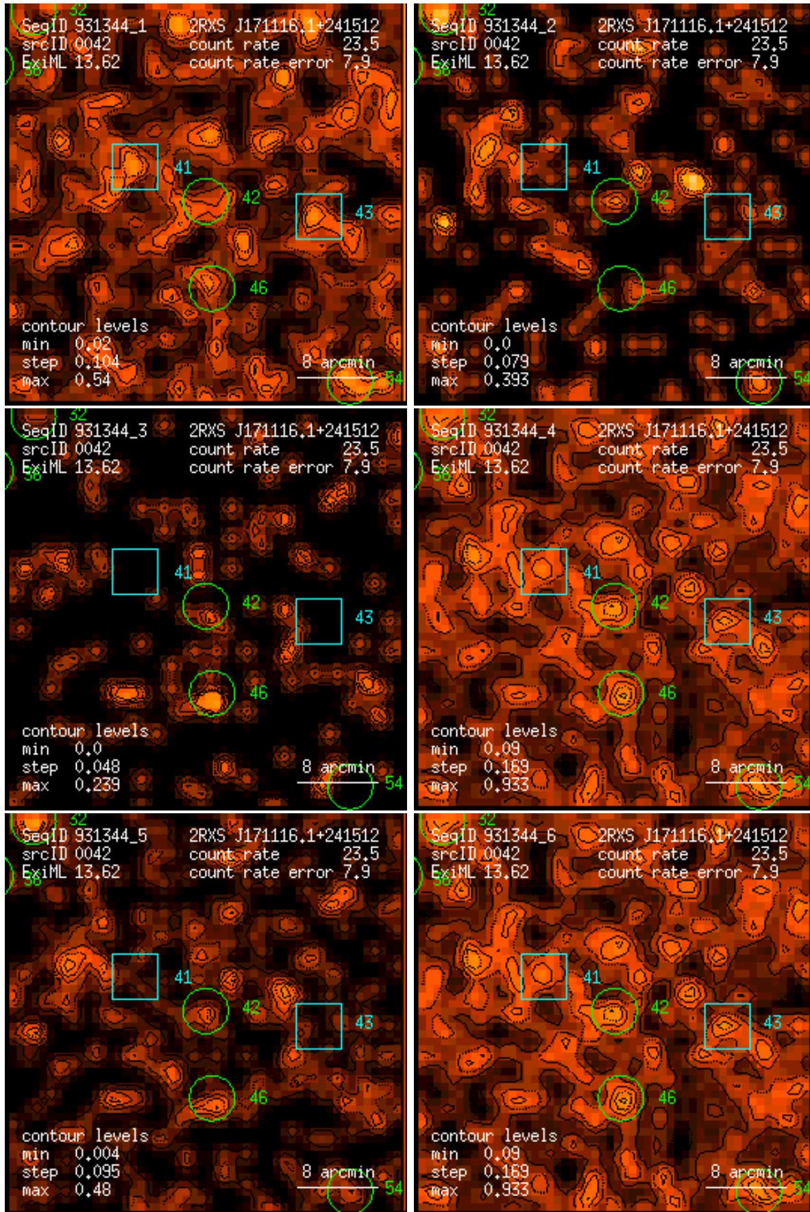
Figure 42: RASS 931344: detection 0042: band rate images, Gaussian filter: (1) PSPC channels 11 – 41, (2) 52 – 90, (3) 91 – 201, (4) 11 – 235, (5) 52 – 201, (6) 11 – 201. Broad band rates in counts/ks. Band rate contour levels in counts/ks/arcmin 2 .
