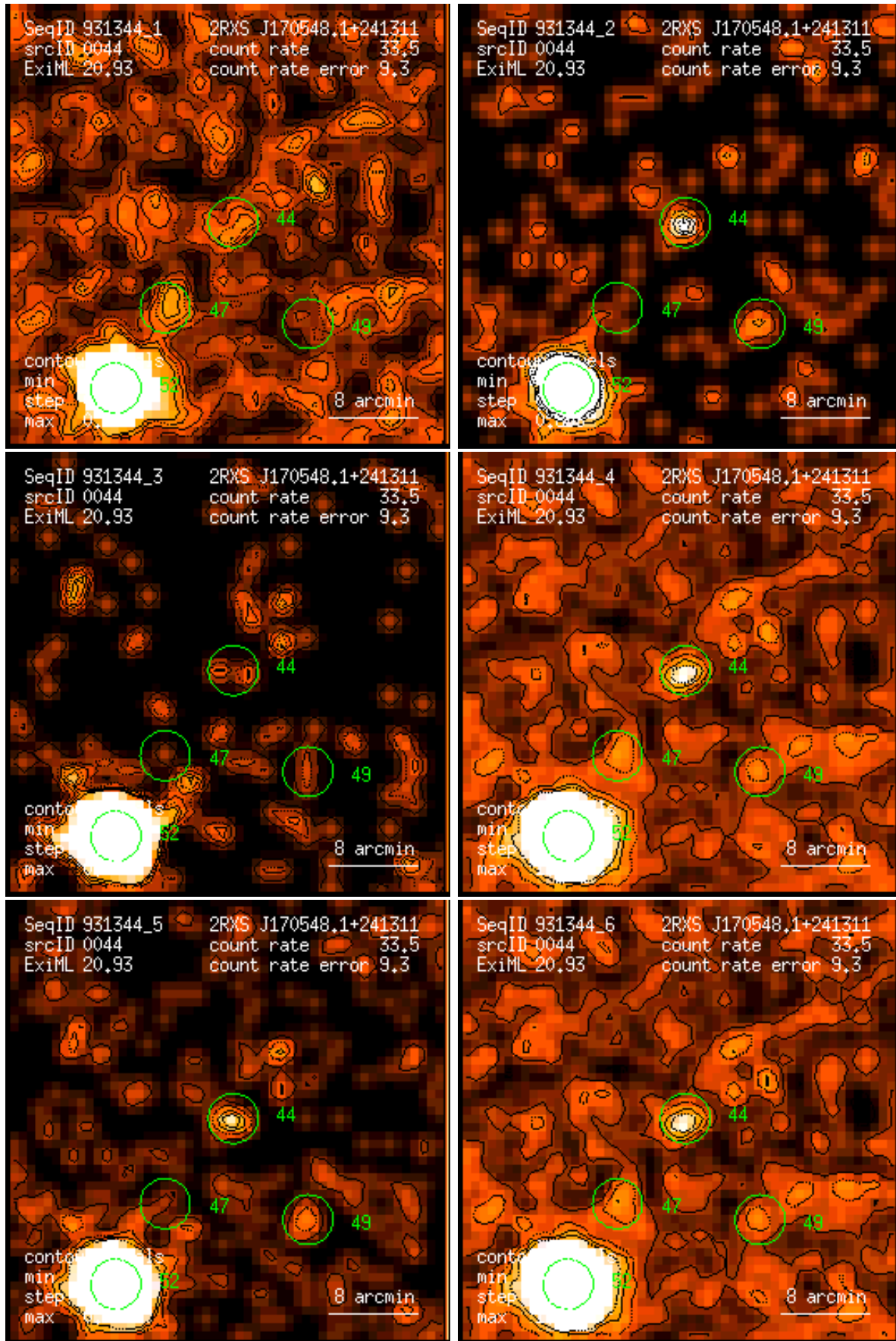
Figure 44: RASS 931344: detection 0044: band rate images, Gaussian filter: (1) PSPC channels 11 – 41, (2) 52 – 90, (3) 91 – 201, (4) 11 – 235, (5) 52 – 201, (6) 11 – 201. Broad band rates in counts/ks. Band rate contour levels in counts/ks/arcmin 2 .
