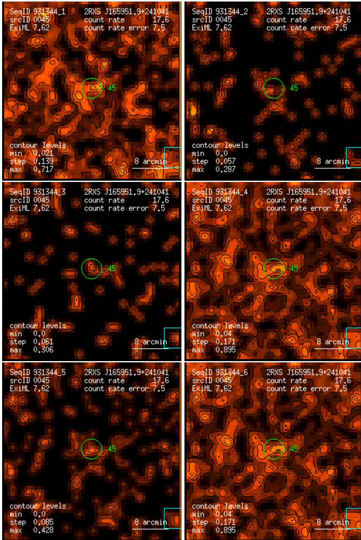
Figure 45: RASS 931344: detection 0045: band rate images, Gaussian filter: (1) PSPC channels 11 – 41, (2) 52 – 90, (3) 91 – 201, (4) 11 – 235, (5) 52 – 201, (6) 11 – 201. Broad band rates in counts/ks. Band rate contour levels in counts/ks/arcmin 2 .
