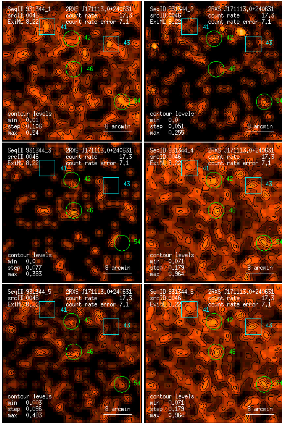
Figure 46: RASS 931344: detection 0046: band rate images, Gaussian filter: (1) PSPC channels 11 – 41, (2) 52 – 90, (3) 91 – 201, (4) 11 – 235, (5) 52 – 201, (6) 11 – 201. Broad band rates in counts/ks. Band rate contour levels in counts/ks/arcmin 2 .
