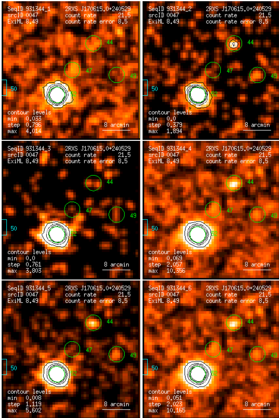
Figure 47: RASS 931344: detection 0047: band rate images, Gaussian filter: (1) PSPC channels 11 – 41, (2) 52 – 90, (3) 91 – 201, (4) 11 – 235, (5) 52 – 201, (6) 11 – 201. Broad band rates in counts/ks. Band rate contour levels in counts/ks/arcmin 2 .
