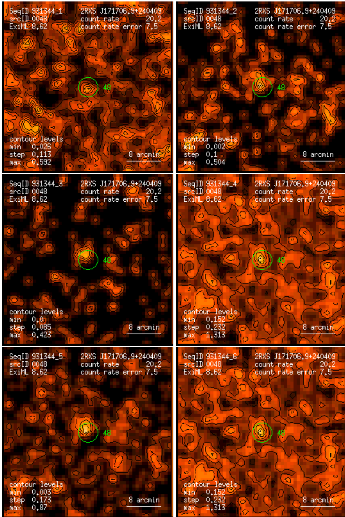
Figure 48: RASS 931344: detection 0048: band rate images, Gaussian filter: (1) PSPC channels 11 – 41, (2) 52 – 90, (3) 91 – 201, (4) 11 – 235, (5) 52 – 201, (6) 11 – 201. Broad band rates in counts/ks. Band rate contour levels in counts/ks/arcmin 2 .
