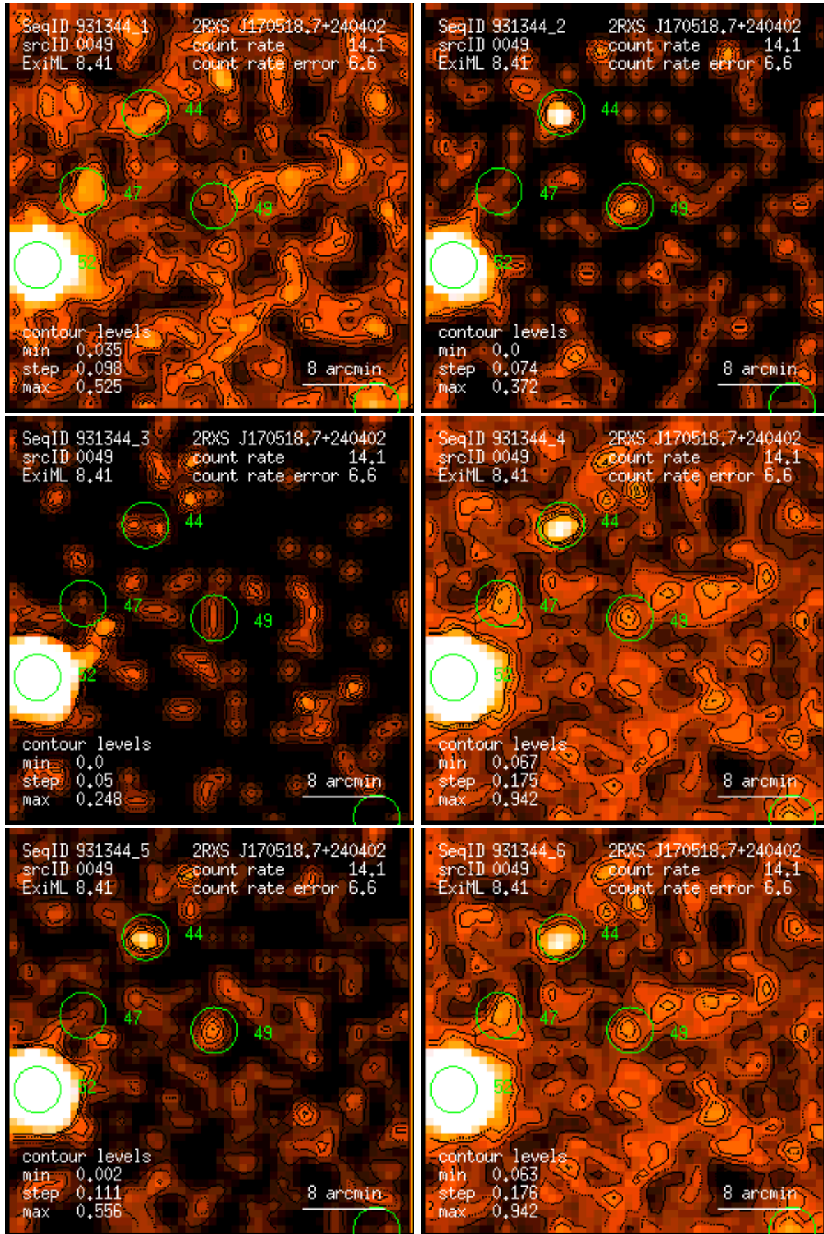
Figure 49: RASS 931344: detection 0049: band rate images, Gaussian filter: (1) PSPC channels 11 – 41, (2) 52 – 90, (3) 91 – 201, (4) 11 – 235, (5) 52 – 201, (6) 11 – 201. Broad band rates in counts/ks. Band rate contour levels in counts/ks/arcmin 2 .
