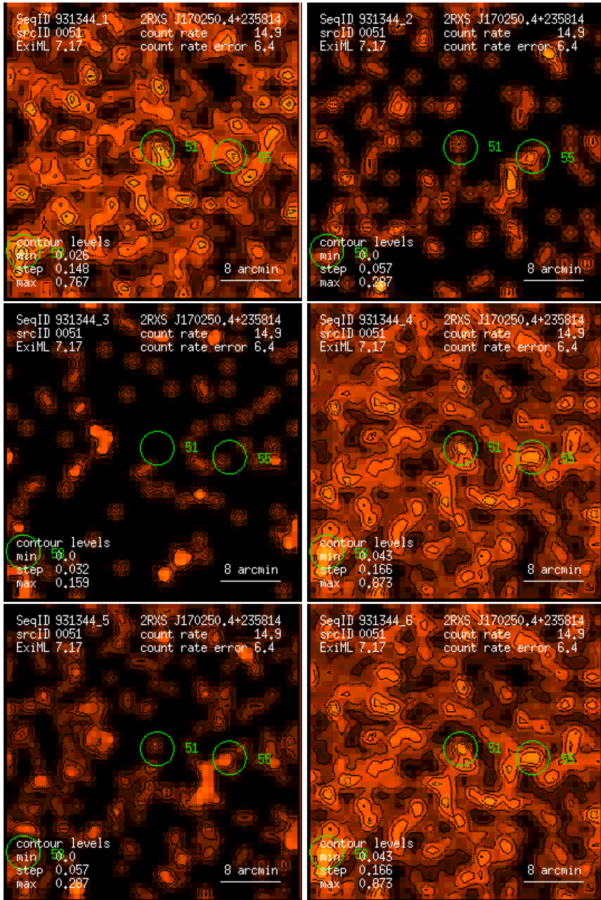
Figure 51: RASS 931344: detection 0051: band rate images, Gaussian filter: (1) PSPC channels 11 – 41, (2) 52 – 90, (3) 91 – 201, (4) 11 – 235, (5) 52 – 201, (6) 11 – 201. Broad band rates in counts/ks. Band rate contour levels in counts/ks/arcmin 2 .
