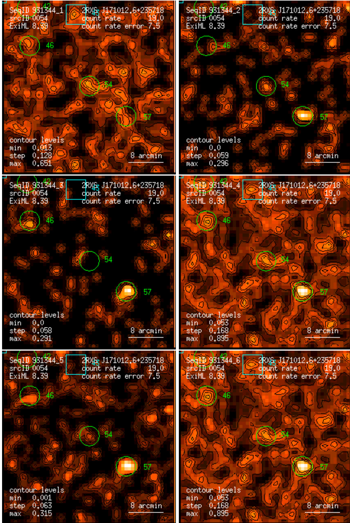
Figure 54: RASS 931344: detection 0054: band rate images, Gaussian filter: (1) PSPC channels 11 – 41, (2) 52 – 90, (3) 91 – 201, (4) 11 – 235, (5) 52 – 201, (6) 11 – 201. Broad band rates in counts/ks. Band rate contour levels in counts/ks/arcmin 2 .
