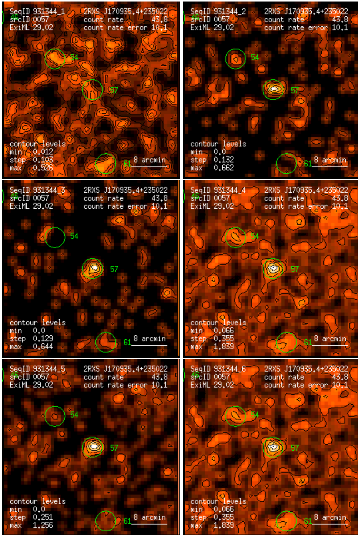
Figure 57: RASS 931344: detection 0057: band rate images, Gaussian filter: (1) PSPC channels 11 – 41, (2) 52 – 90, (3) 91 – 201, (4) 11 – 235, (5) 52 – 201, (6) 11 – 201. Broad band rates in counts/ks. Band rate contour levels in counts/ks/arcmin 2 .
