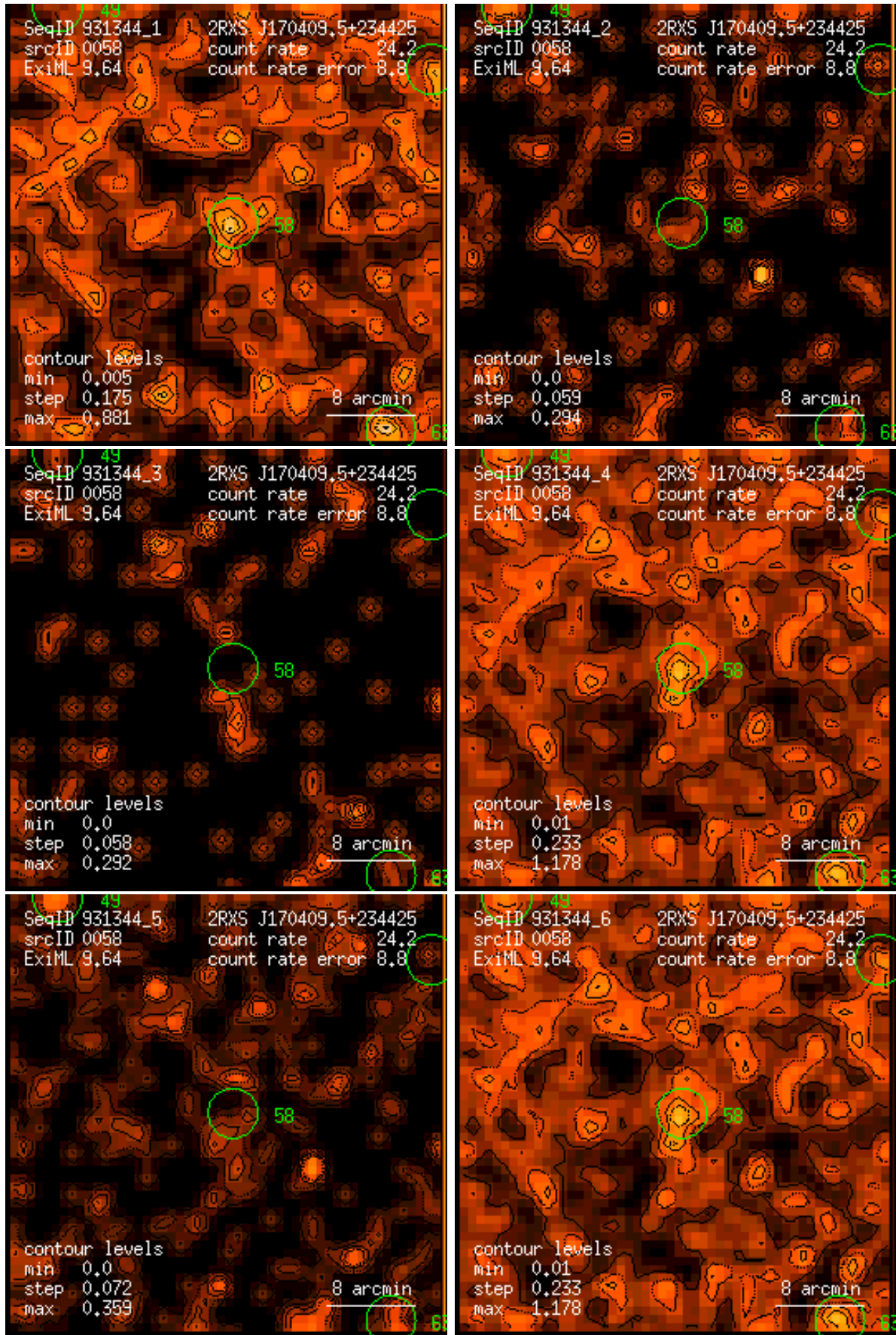
Figure 58: RASS 931344: detection 0058: band rate images, Gaussian filter: (1) PSPC channels 11 – 41, (2) 52 – 90, (3) 91 – 201, (4) 11 – 235, (5) 52 – 201, (6) 11 – 201. Broad band rates in counts/ks. Band rate contour levels in counts/ks/arcmin 2 .
